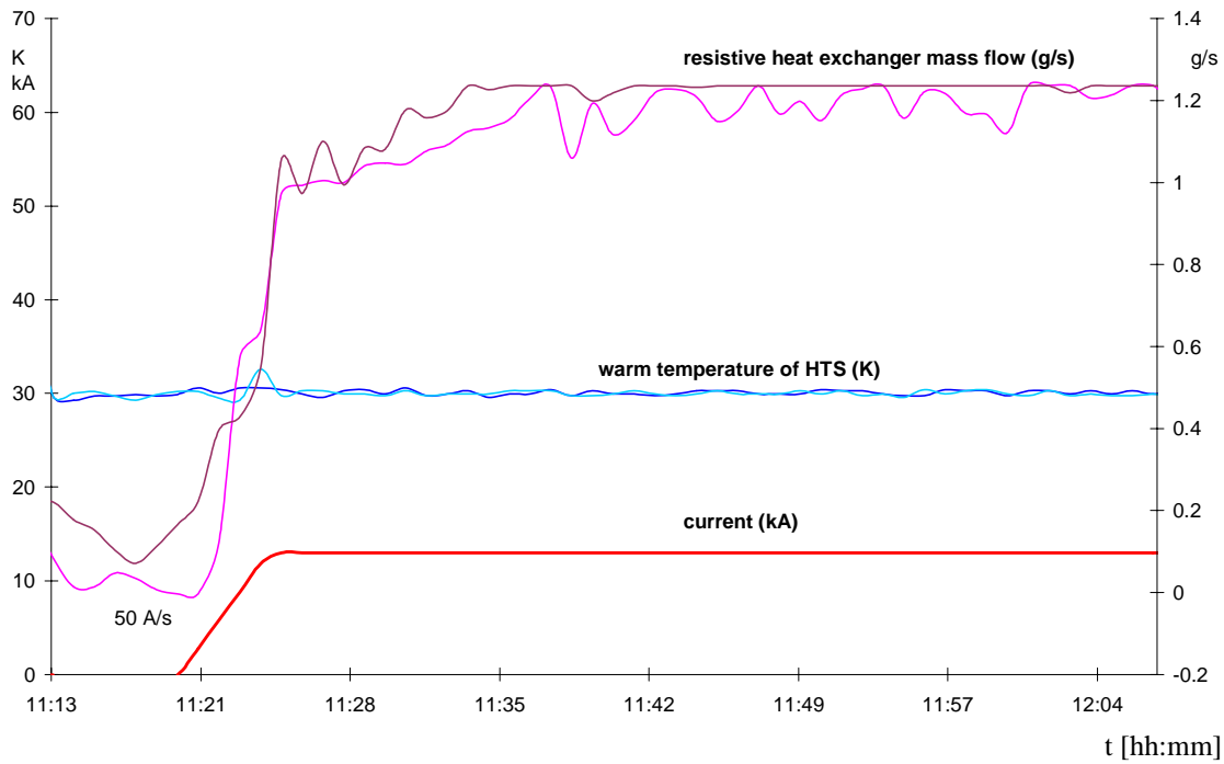
Figure 5. Typical response of cryogenic parameters during current ramping of leads.
