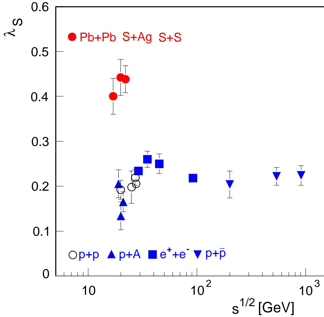
Figure 10: Strangeness suppression factor ( \lambda_S = \langle s + \bar{s} \rangle / (\langle u + \bar{u} \rangle + \langle d + \bar{d} \rangle) ) as a function of c.m. collision energy for different types of high energy interactions.
