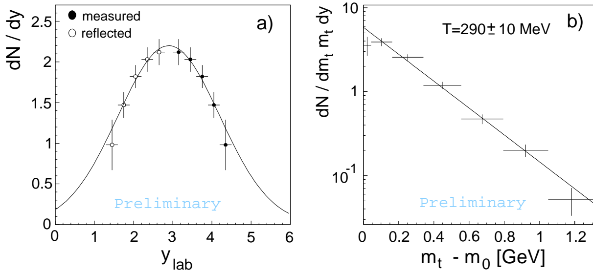
Figure 16: a) y and b) p_T distribution of \Phi produced in central Pb+Pb interactions.
