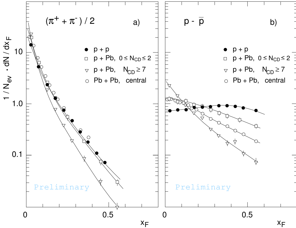
Figure 7: x_F distributions for a) mean charged pions and b) participating protons observed in p+p , peripheral and central p+Pb , as well as central Pb+Pb collisions. The central Pb+Pb results are scaled down by 176 (assumed number of participant nucleon pairs [7]).
