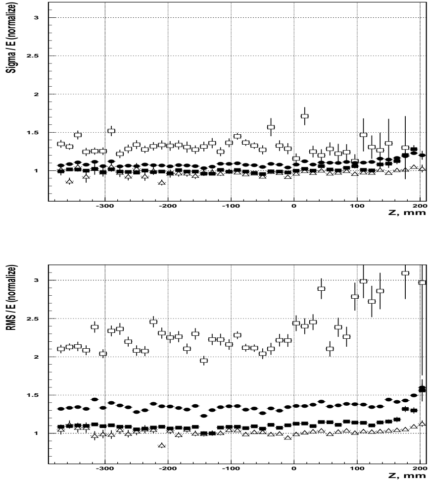
Figure 11: Normalised energy resolutions ( \sigma/E_G ) obtained by Gaussian fitting (top) and normalised energy resolutions ( RMS/ \langle E \rangle ) obtained by averaging of spectrum (bottom) as a function of Z coordinate at different leakage conditions: a) black square — no leakage, b) open square — longitudinal leakage, c) open triangle — lateral leakage, d) black circle — all events.
