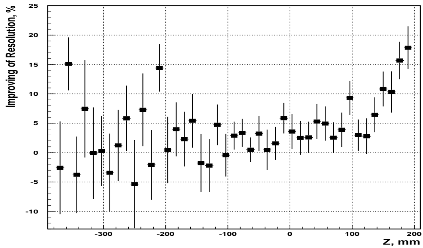
Figure 12: The lateral leakage (top) and the energy resolution improving (bottom) for the events sample with lateral leakage as a function of Z coordinate.
