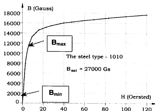
Figure 1: B versus H for the low-carbon steel (1010)
