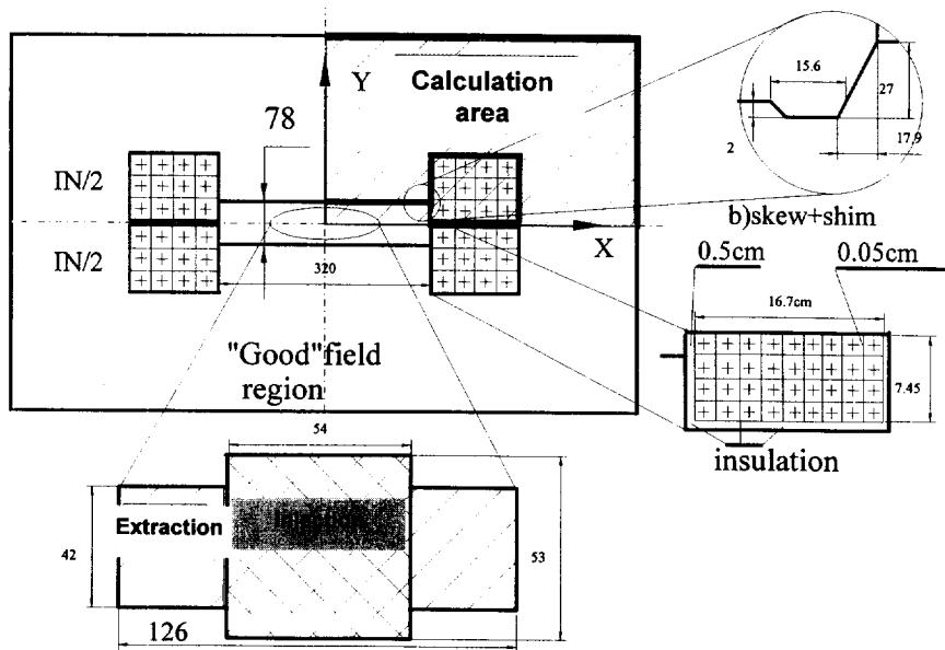
Figure 3: General layout of the dipole magnet cross section.
