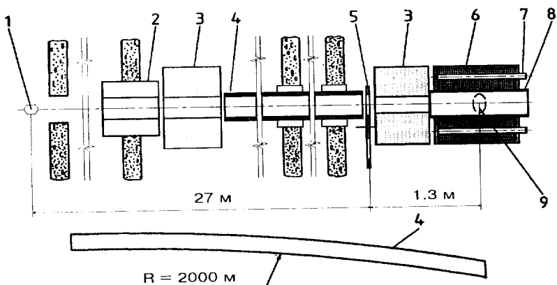
Fig. 1 The scheme of the "Isomer" setup: 1- IBR-2 reactor active zone and the moderator; 2,3 - collimators; 4 - bent mirror guide; 5 - chopper; 6- neutron detector; 7 - ^3\text{He} -counters; 8 - Cd tube; 9 - sample.
