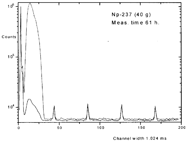
Fig. 5. The experimental spectrum for ^{237}\text{Np} . The channel width is equal to 1.024 ms.
