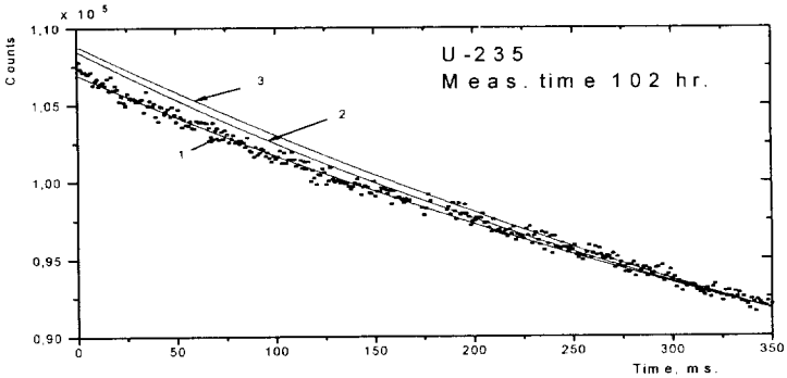
Fig. 6. The experimental DN decay curve for ^{235}\text{U} and the calculated ones using different 6-group sets of constants: 1- Keepin-Tuttle [1,2]; 2 - Waldo et al. [23]; 3 - Mills et al. [24].
