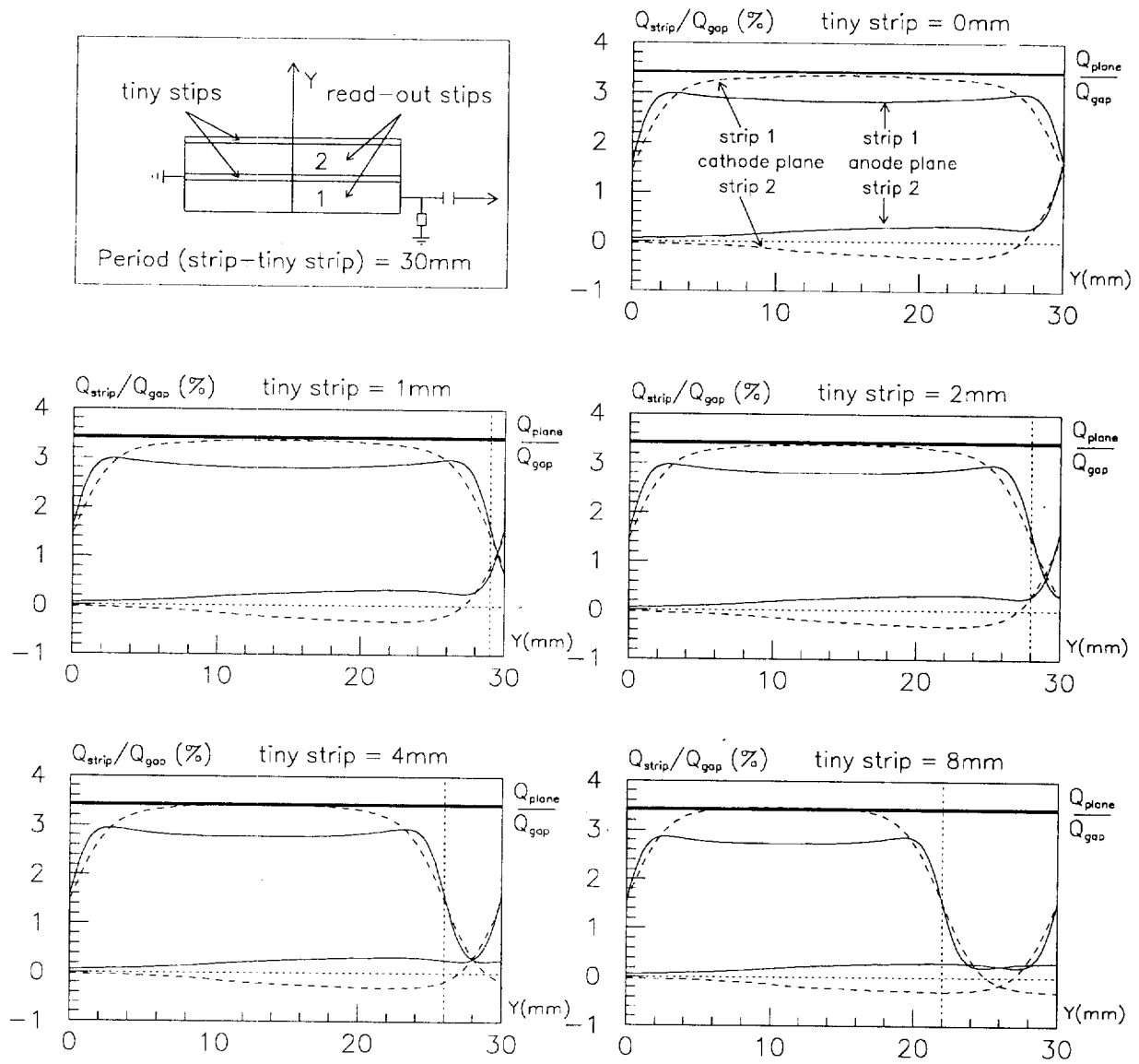
Fig. 8. Read-out strip charges in dependence on avalanche position. Unbroken foil coating. Electrode \epsilon=4 .
