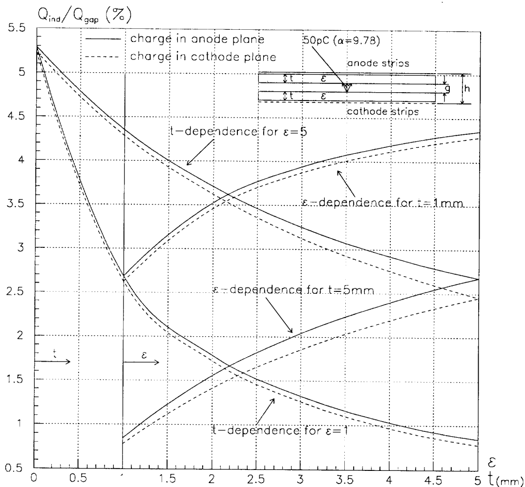
Fig. 4. Induced charge in dependence on electrode permittivity ( \epsilon ) and thickness ( t ). Gap ( g ) is fixed 2mm.
