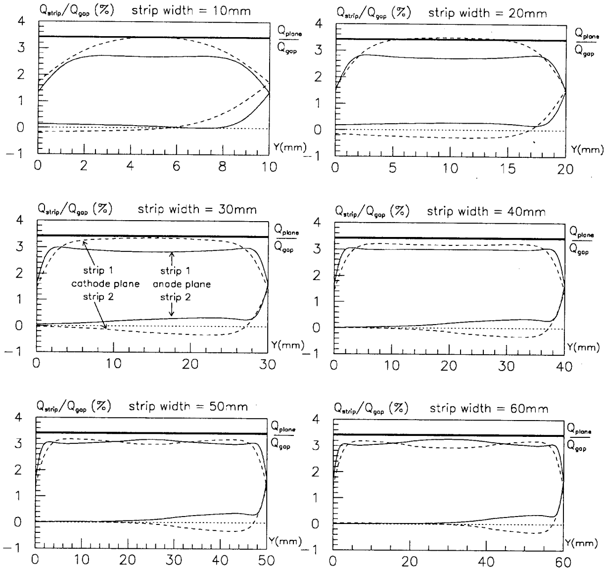
Fig. 10. Read-out strip charges in dependence on avalanche position for different strip width. Electrode \epsilon=4 .
