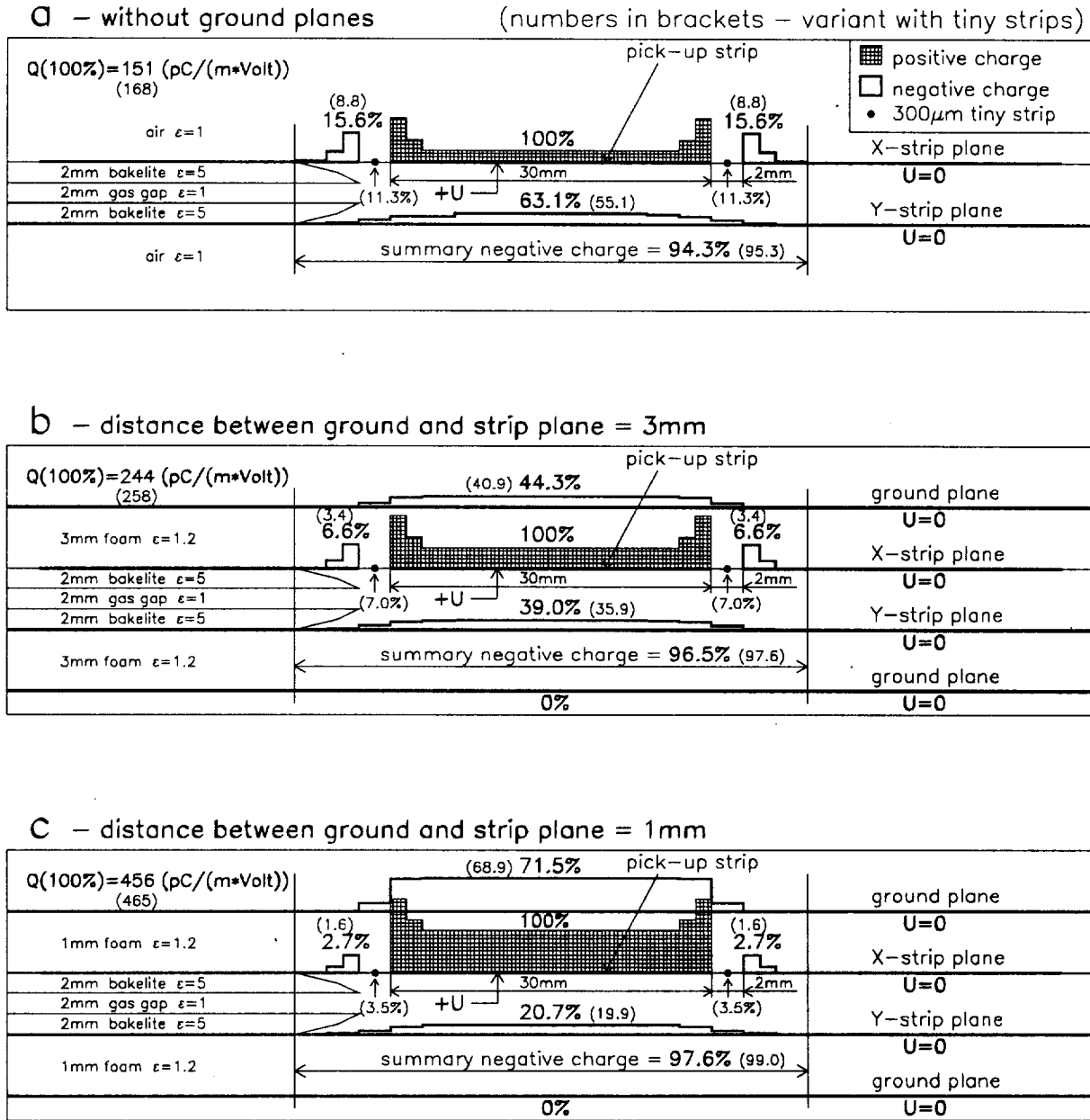
Fig. 13. Charge density distribution due to capacitance coupling. Charge density in arbitrary scale.
