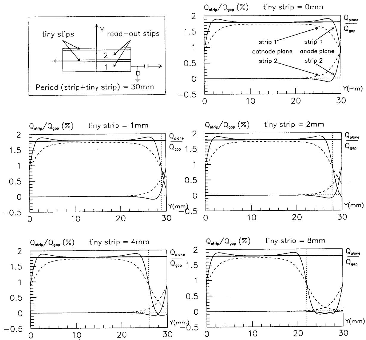
Fig. 7. Read-out strip charges in dependence on avalanche position. Unbroken foil coating. Electrode \epsilon=1 .
