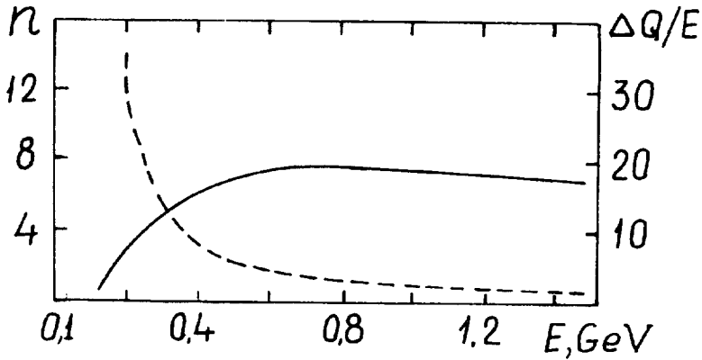
Fig. 1. Dependence of the relative energy gain \Delta Q = |Q(E) - E|/E (solid curve) and the correction factor of proton current n(E) (dashed curve) on the bombarding proton energy E . The calculation have been done for the electronuclear system designed in JINR on the basis of the core of the impulse plutonium reactor IBR-30 [2, 3]. Coefficient of neutron multiplication K_{eff} = 0.943 \pm 0.003 .
