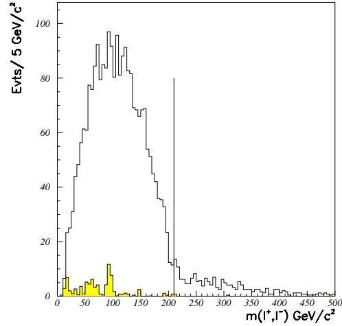
Figure 21: CM S dilepton invariant mass distribution for \kappa_{121} = 0.05, m_0 = 1000, m_{12} = 500, \tan \beta = 2, A_0 = 0 and \mu < 0 . The shaded area corresponds to the SM background. The straight line indicates the \tilde{m}_1^0 mass equal to 210 \text{ GeV}/c^2 . Signal and background are normalized to an integrated luminosity of 10^4 \text{ pb}^{-1} .
