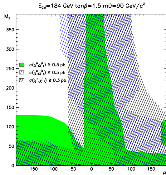
Figure 15: Gaugino cross sections in the (\mu, M_2) plane for \tan\beta = 1.5 , m_0 = 90 \text{ GeV} = c^2 and \sqrt{s} = 184 \text{ GeV} ; in the dark grey area (e^+ e^- \rightarrow e_1^0 e_1^0) > 0.3 \text{ pb} , in the hatched area (e^+ e^- \rightarrow e_2^0 e_1^0) > 0.3 \text{ pb} and/or (e^+ e^- \rightarrow e_1^+ e_1^-) > 0.3 \text{ pb} .
