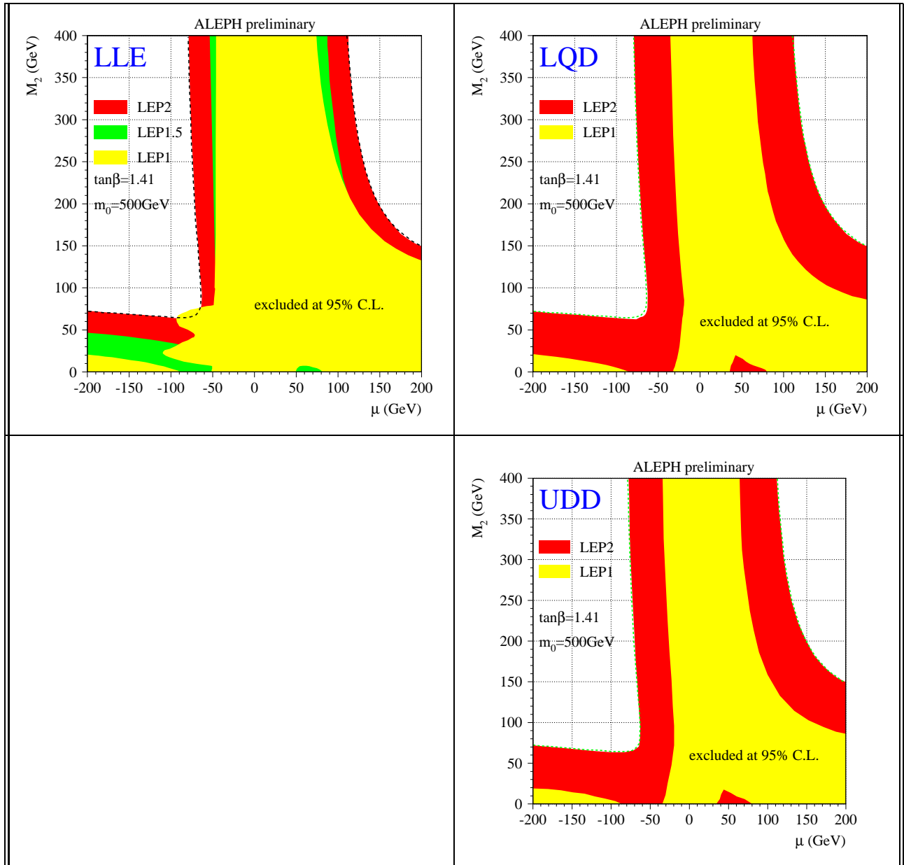
Figure 11: Charginos and Neutralinos 95 % C.L. exclusion in the \mu, M_2 plane for \tan\beta = 1.41 . Valid for any choice of generation indices i, j, k of the couplings \lambda_{ijk}^0 and \lambda_{ijk}^\infty and valid for m_0 = 500 \text{ GeV} = c^2 i.e. large sfermion masses.
