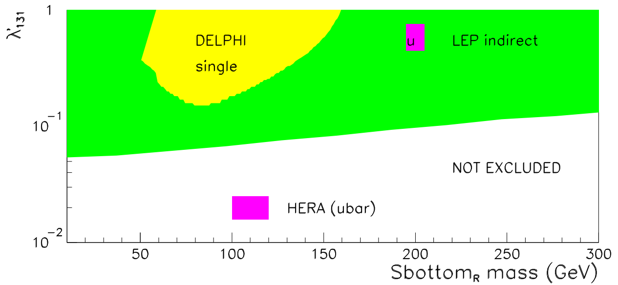
Figure 13: Exclusion domain in the \lambda_{131-132} versus m_{\tilde{q}} plane.
