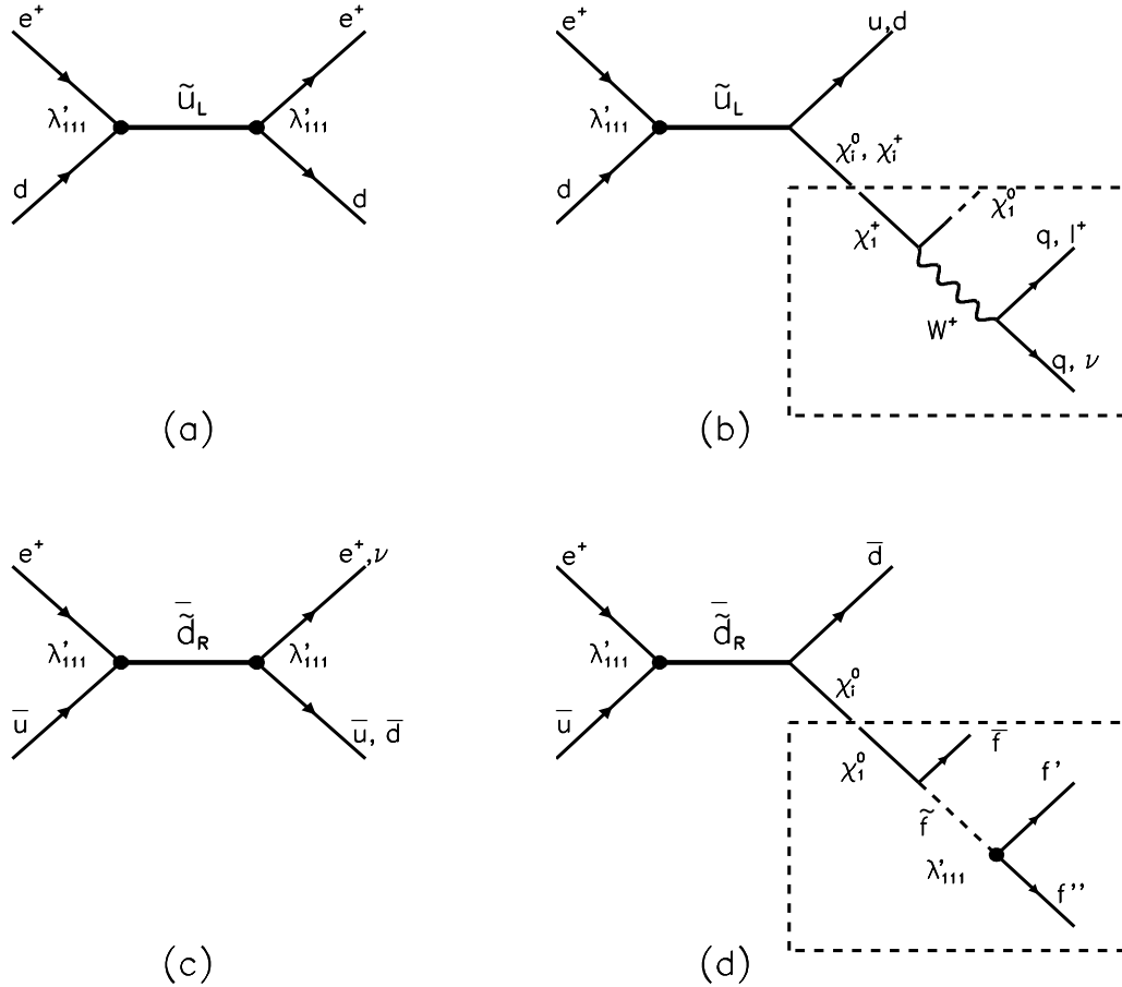
Figure 3: Lowest order s-channel diagrams for first generation squark production at HERA followed by (a),(c) \mathbb{R}_p decays and (b),(d) gauge decays. In (b) and (d), the emerging neutralino or chargino might subsequently undergo \mathbb{R}_p decays of which examples are shown in the dotted boxes for (b) the \chi_1^+ and (d) the \chi_1^0 .
