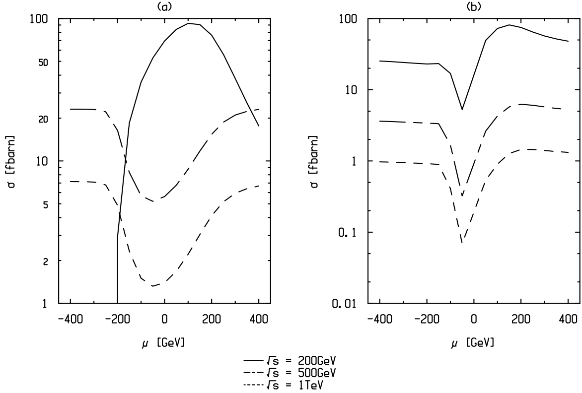
Figure 1: The cross sections for the processes e^+e^- \rightarrow \tilde{\chi}^0_1 \tilde{\chi}^0_1 (a) and e^+e^- \rightarrow \tilde{\chi}^0_1 \tilde{\chi}^0_2 (b), as a function of \mu , using the set of parameters: M_2 = 200\text{ GeV} , m_0 = 150\text{ GeV} , m_{11} = 0.05 and \tan\beta = 2 . The different center of mass energies are indicated under the figures.
