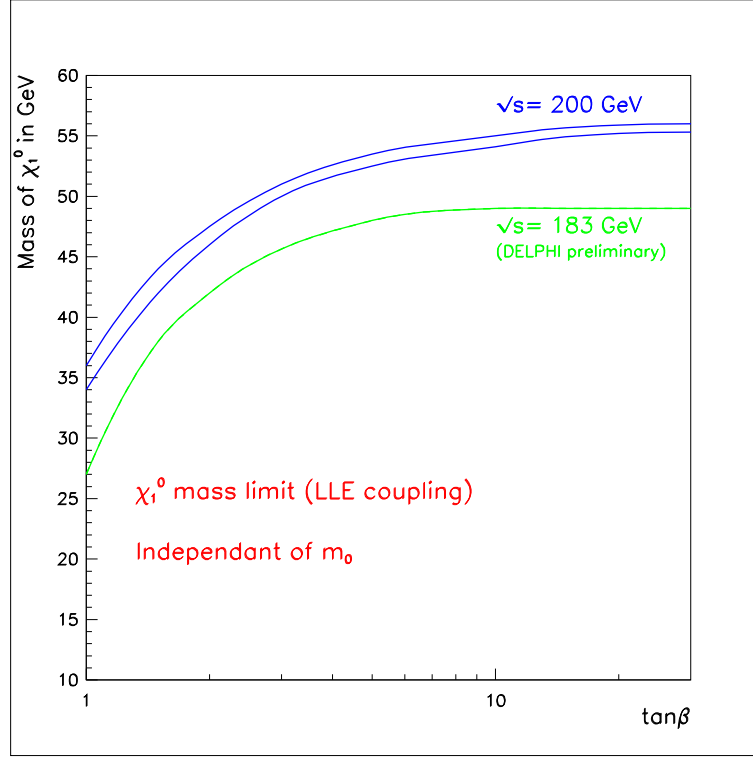
Figure 17: \chi_1^0 mass limit as a function of \tan\beta . The light grey curve presents the preliminary current limit obtained by DELPHI with the 1997 data. The 2 dark grey curves show the range for the expected \chi_1^0 mass limit in case of 200 pb -1 collected at \sqrt{s} = 200 GeV: the upper curve is obtained assuming N_{95} = 5 , \tilde{\nu}_1^0\tilde{\nu}_1^0 = 30\% , \tilde{\nu}_2^0\tilde{\nu}_1^0 = 20\% , \tilde{\nu}_1^+\tilde{\nu}_1^- = 25\% ; the lower curve is obtained assuming N_{95} = 15 , \tilde{\nu}_1^0\tilde{\nu}_1^0 = 30\% , \tilde{\nu}_2^0\tilde{\nu}_1^0 = 25\% , \tilde{\nu}_1^+\tilde{\nu}_1^- = 15\%
