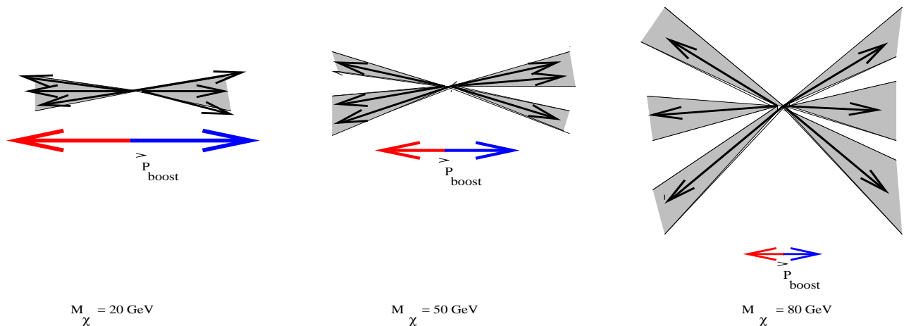
Figure 10: Schematic jet patterns for the 6-quarks partonic final states of neutralino pair decay with \tilde{g}_{ijk}^0 couplings.
