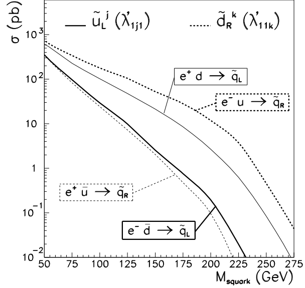
Figure 2: Squark production cross-sections in ep collisions for a coupling \lambda_0 = 0.1 .
