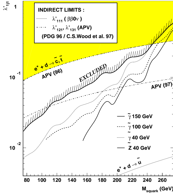
Figure 5: Exclusion upper limits at 95% C.L. for the coupling \lambda'_{1j1} as a function of squark mass, for various masses of a \tilde{\chi}_1^0 -like \tilde{\chi}_1^0 ; the difference obtained between a 40 GeV \tilde{\chi}_1^0 -like and Z -like \tilde{\chi}_1^0 is also shown; also represented are the most stringent indirect limits on \lambda'_{111} and \lambda'_{1j1} , j = 2;3 .
