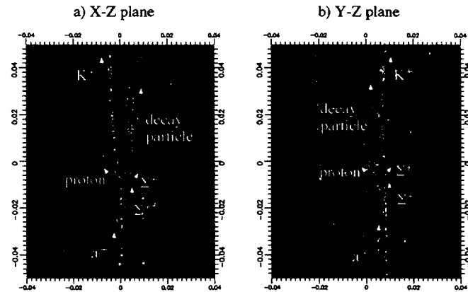
Figure 5: Pictures of a typical event finally identified as \Sigma^+p scattering. The images on the a) X-Z plane and b) Y-Z plane are shown.
