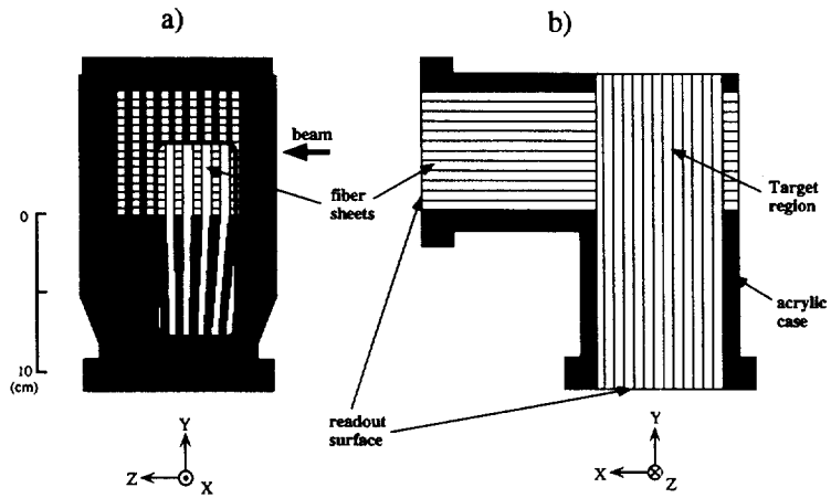
Figure 2: Schematic view of the SCIFI target. a) view from the horizontal I.I.T. b) view from the upstream.
