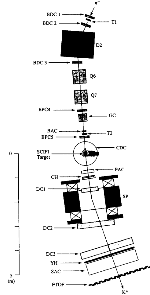
Figure 1: Top view of the experimental setup.
