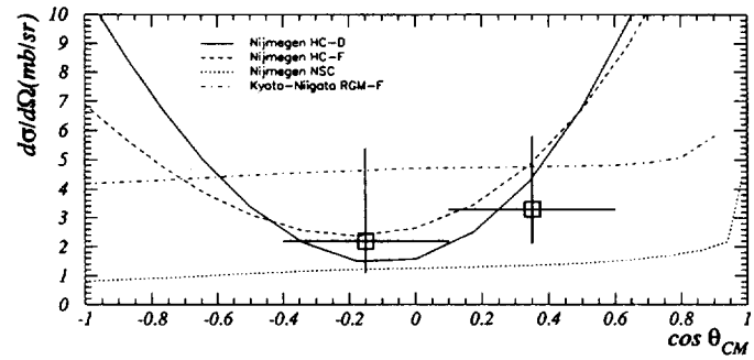
Figure 6: Comparison of the measured differential cross sections for \Sigma^+p \rightarrow \Sigma^+p with theoretical calculations by the Nijmegen group with the hard-core models D (HC-D), F (HC-F), and the soft-core model (NSC) [12] and by the Kyoto-Niigata group with the quark-cluster model (RGM-F) [13] at the \Sigma^+ momentum of 400 MeV/c.
