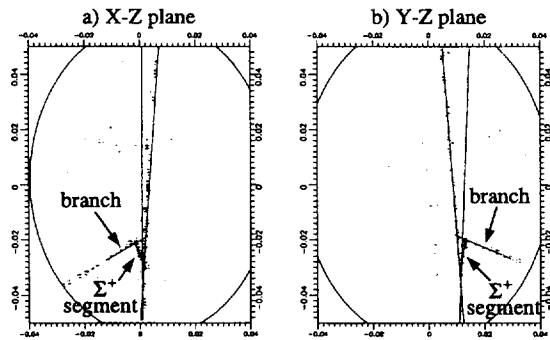
Figure 3: An example of the result of the automatic-tracking process for the real image data. The images on the a) X-Z plane and b) Y-Z plane are shown.
