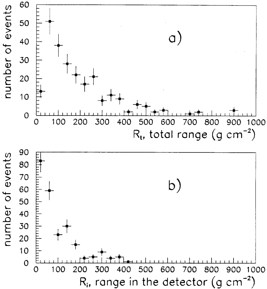
Figure 4: a) Distribution of the reconstructed total range R_t of the up-going particles for which |z_v^w - z_v^s| < 50\ cm . Events with a poorly reconstructed vertex are excluded from this distribution because of the large uncertainty in R_t for these events. b) Distribution of the grammage traversed in the detector, R_i , for all the 243 up-going particles in the final data set.
