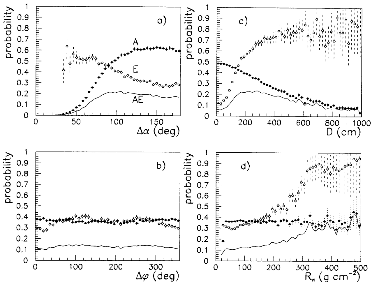
Figure 6: Distribution of the probability A for events to be accepted, of the tracking efficiency E , and of the reconstruction efficiency AE versus (a) \Delta\alpha , (b) \Delta\phi , (c) D , and (d) R_\pi . Each quantity is averaged over the three remaining variables. Full points: A ; empty points: E ; solid curves: AE .
