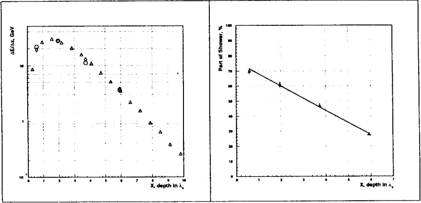
Figure 11: Left: Longitudinal profile as a function of longitudinal coordinate x in units \lambda_{\pi}^{Fe} . Open circle - our data, open triangle — data for conventional calorimeter, diamond - Monte Carlo prediction. Right: The fractions of the “electromagnetic” parts of showers in various depths as a function of x .
