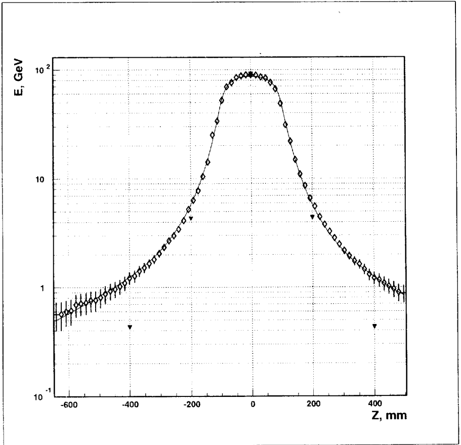
Figure 4: The energy depositions in towers summed overall calorimeter depths as a function of Z coordinate. Curve is the result of fit by formula (14) and (15). Open circles are the Monte Carlo predictions (GEANT-FLUKA+GHEISHA) from Table 3.
