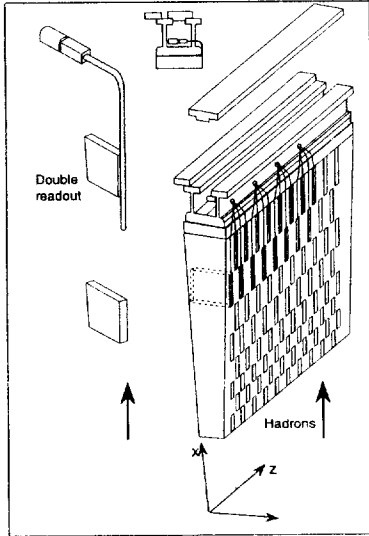
Figure 1: Principle of the tile hadronic calorimeter.
