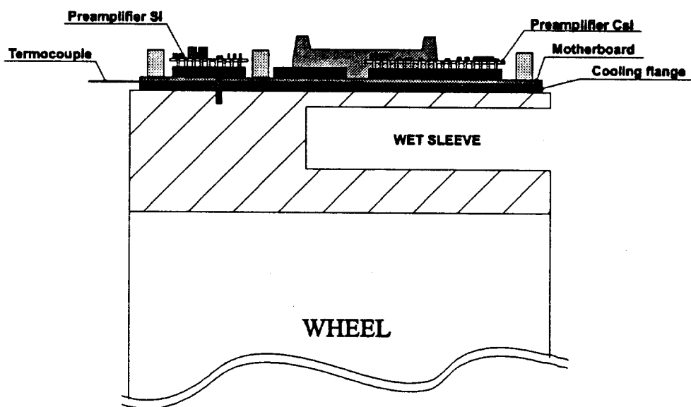
Figure 3-a : Setup for the measurement of the temperature of the motherboard T_{M.B.} .
