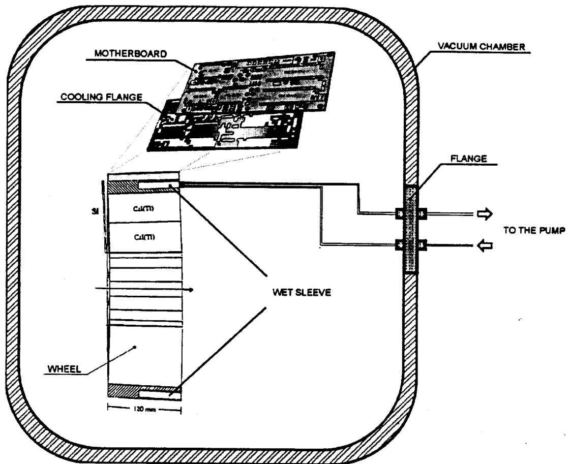
Figure 1 : General assembly scheme of the system under test.
