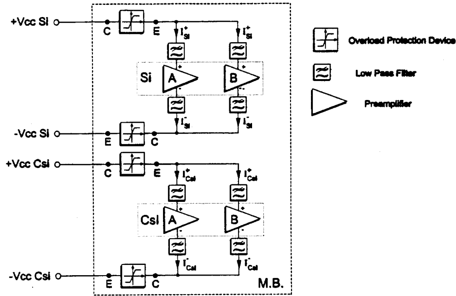
Figure 2 : Motherboard block diagram.
