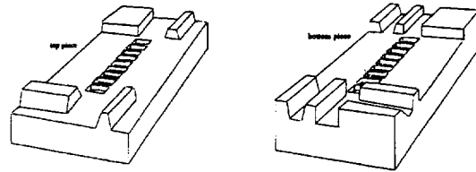
Fig. 6 RF structure halves showing alignment features. (Structure is an accelerator section). 3
