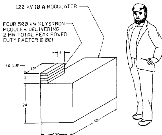
Fig. 9 2-MW, four-module "brick" with estimated modulator dimensions
