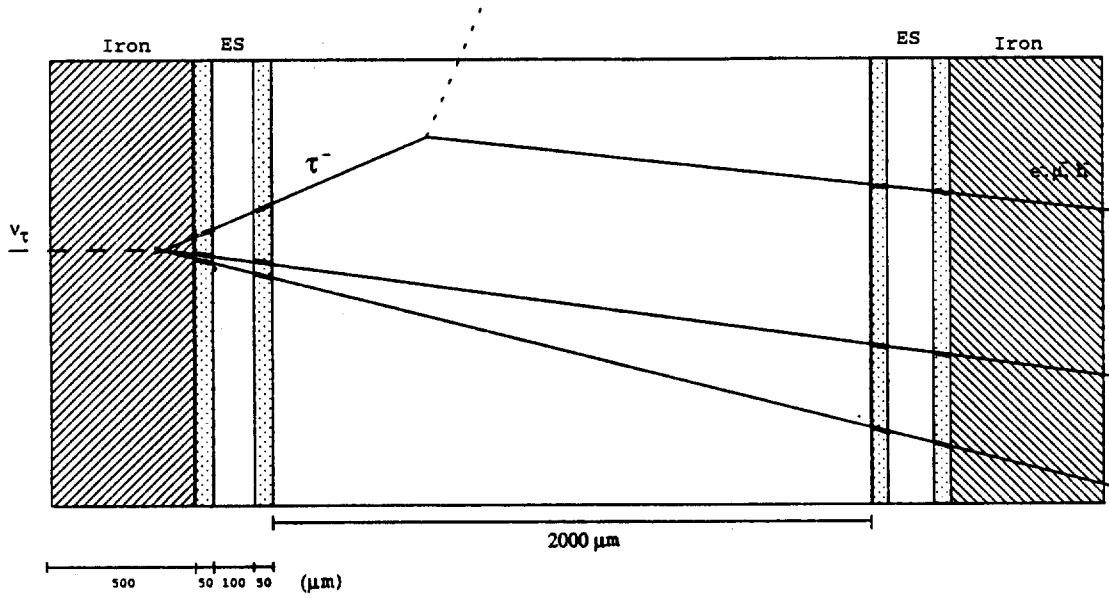
Figure 2: Schematic structure of the OPERA target.
