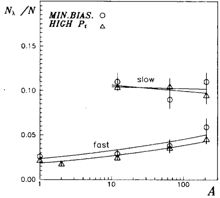
Fig.5: A dependence of ratios \langle N_\Lambda \rangle / \langle N_{slow} \rangle , \langle N_\Lambda \rangle / \langle N_{fast} \rangle , \langle N_{KK} \rangle / \langle N_{slow} \rangle , \langle N_{KK} \rangle / \langle N_{fast} \rangle .
