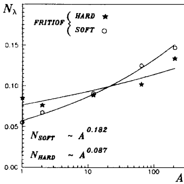
Fig.6: A-dependence of the neutral strange particle production ratio in soft and hard interactions within FRITIOF-7.02.
