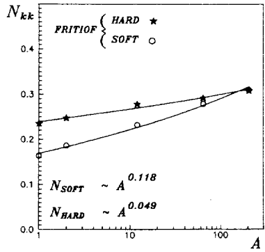
Fig.6: A-dependence of the neutral strange particle production ratio in soft and hard interactions within FRITIOF-7.02.
