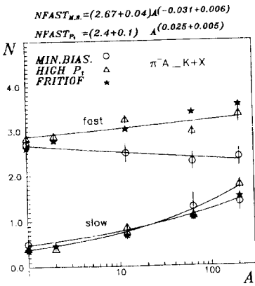
Fig.4: A-dependence of associated negative particle multiplicity.
