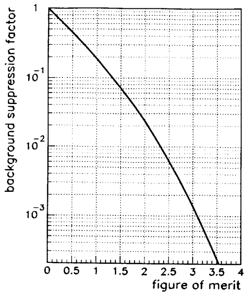
Fig.8. The background suppression factor vs 'figure of merit' f .
