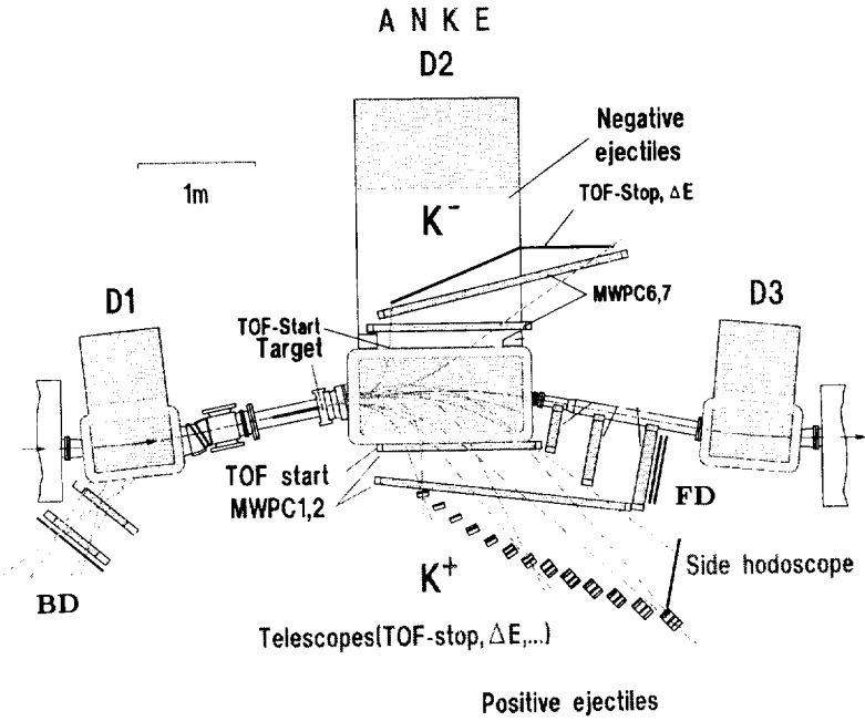
Fig.1. Layout of the experimental setup.
