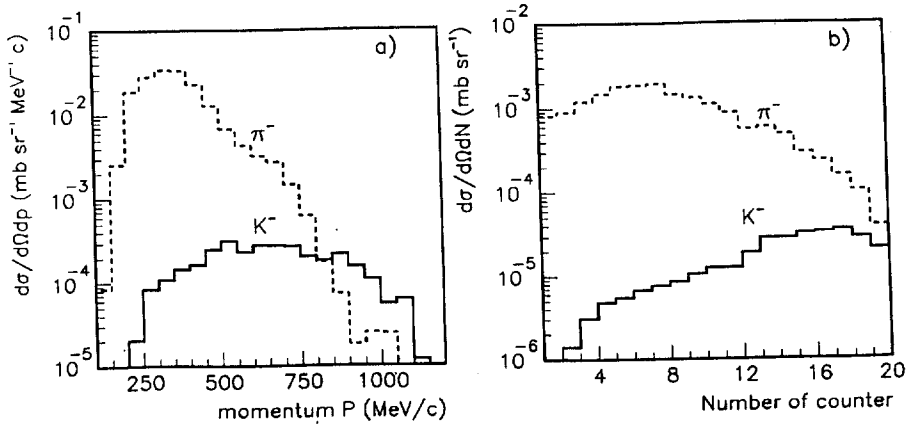
Fig.2. Simulation of negative particle distributions from the reaction p(2500 \text{ MeV}) + {}^{12}\text{C} \rightarrow K^+ + K^- (\pi^-) + X . (a) Momentum spectra of detected particles and (b) distribution of particles detected in Negative side hodoscope vs the module number.
