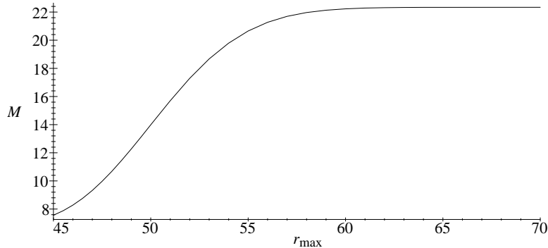
FIG. 9. The mass of the gravitational field of massless NGT as a function of the outer grid point, r_{\max} , for the initial conditions \gamma^{11} = 1 , \psi = A[r/r_0]^2 e^{-(r-r_0)^2/\sigma^2} , and j^2_3 = 0 , where A = 0.7 , and with \sigma = 10 in units where r_0 = 40 .
