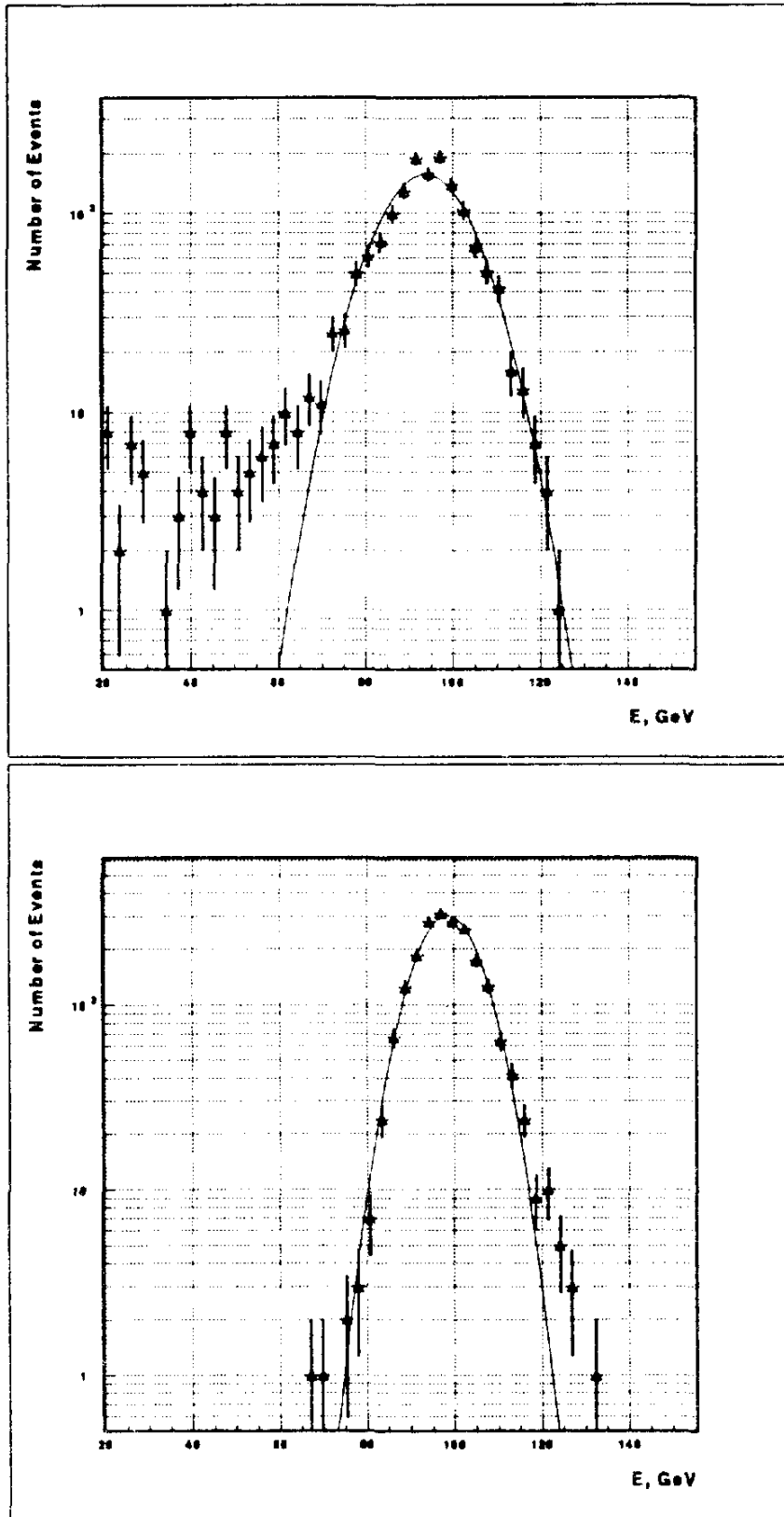
Figure 8: Energy responses for all Z = -8 \text{ cm} at a different leakage conditions: longitudinal leakage (top), lateral leakage (bottom).
