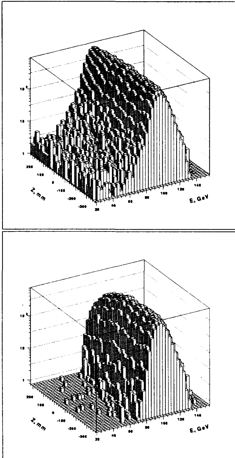
Figure 3: Two dimensional spectrum of energy response as a function of Z coordinate and energy E for various leakage conditions: all events (top), no leakage (bottom).
