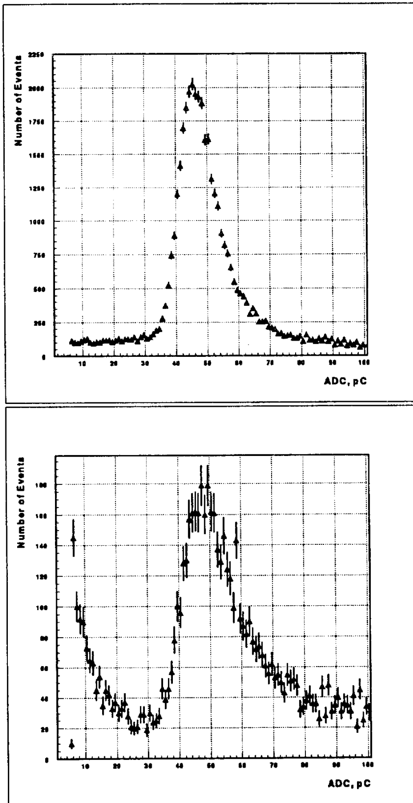
Figure 2: Typical ADC spectrum of a “muon wall” counters in the \mu beam (top) and in the \pi beam (bottom) for counter N^Q 8.
