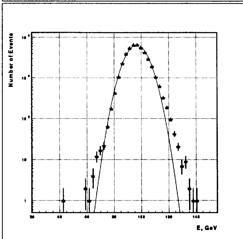
Figure 6: Energy responses for Z at a different leakage conditions: longitudinal leakage (top), lateral leakage (bottom).
