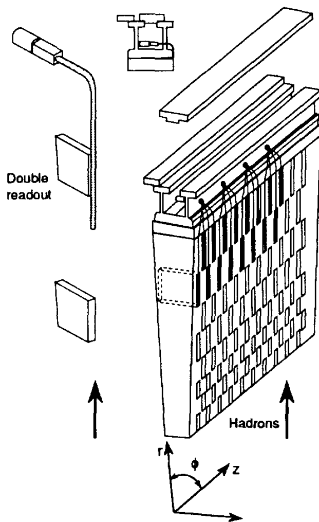
Figure 1: Principle of the tile hadronic calorimeter.
