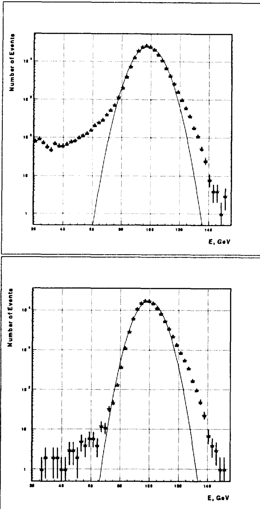
Figure 5: Energy responses for all Z at a different leakage conditions: all events (top), no leakage (bottom).
