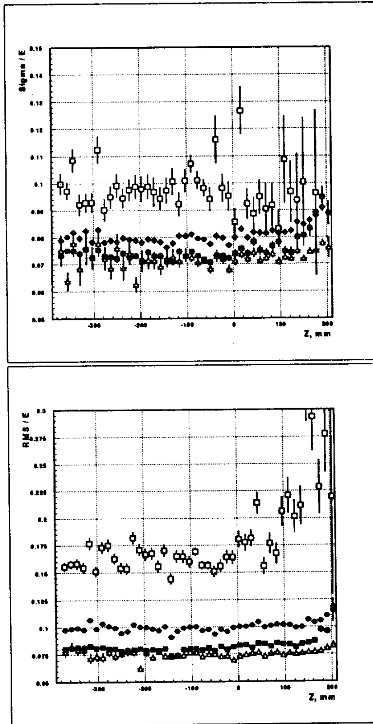
Figure 10: Energy resolutions ( \sigma/E_G ) obtained by Gaussian fitting (top) and energy resolutions ( RMS/ \langle E \rangle ) obtained by averaging of spectrum (bottom) as a function of Z coordinate at different leakage conditions: a) black square — no leakage, b) open square — longitudinal leakage, c) open triangle — lateral leakage, d) black circle — all events.
