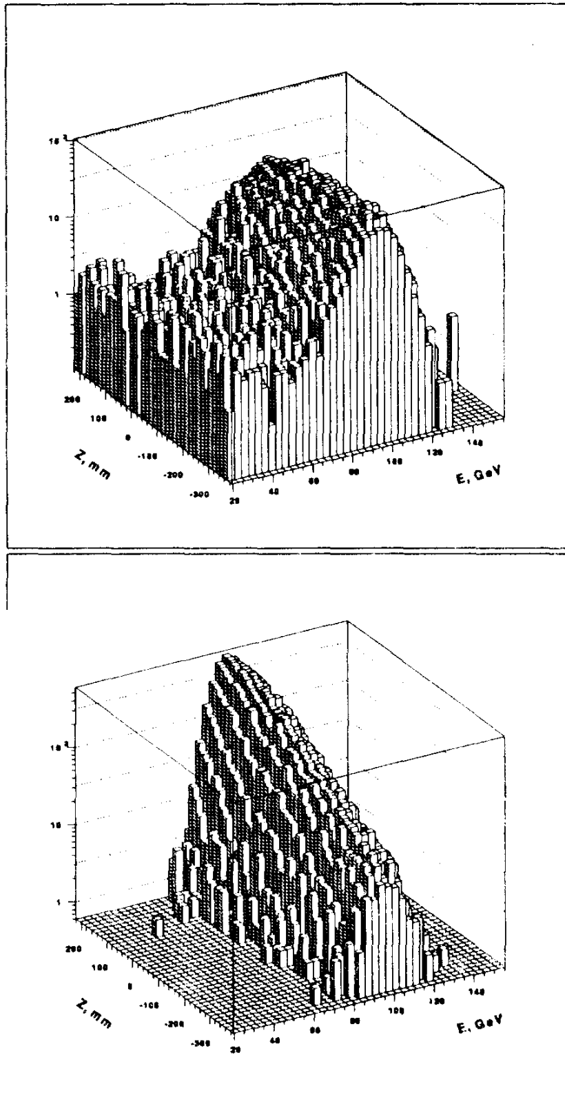
Figure 4: Two dimensional spectrum of energy response as a function of Z coordinate and energy E for various leakage conditions: longitudinal leakage (top), lateral leakage (bottom).
