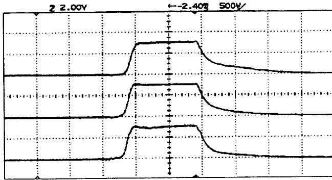
Fig. 7. Ion current from the three probes at 450 V across 100 k \Omega resistors: center probe (bottom), probe at 3 cm radius (middle), probe at 6 cm radius (top).
