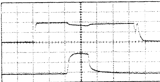
Fig. 8. The effect of insufficient capacitance on bias voltage (top). (The lower trace is that of total ion current to the wafer holder.)
