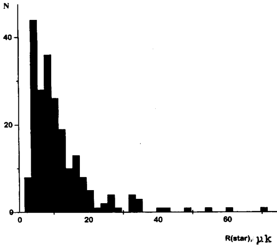
Figure 3a. Distribution of the “stars” number according to the radius R of each “star”.
