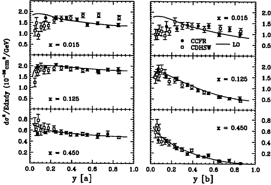
Figure 2: Preliminary differential cross section (statistical error only) for neutrino[a] and antineutrino[b] at E_\nu = 150 GeV: Preliminary CCFR data (solid circles) are compared to the QCD LO prediction and previous CDHSW data (open squares).
