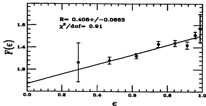
Figure 3: F(x, Q^2, \epsilon) vs \epsilon fit at x = 0.045 and Q^2 = 5.01 \text{ GeV}^2 : The errors on F are only statistical errors.
