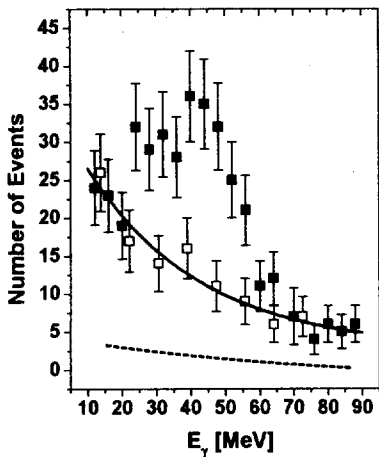
Figure 4: The photon energy spectra for the S_1 \gamma -ray detector. The solid squares correspond to the target filled with liquid hydrogen and the open squares to the empty one. The solid line represents an exponential fit to the empty target data points. The dashed line shows the background of accidental coincidences.
