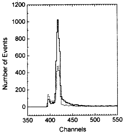
Figure 2: The spectrum of the time of the RF signals with respect to the signal from central detector. The solid and the dotted lines correspond to the target filled with liquid hydrogen and the empty one, respectively. One channel equals 1.0 ns.
