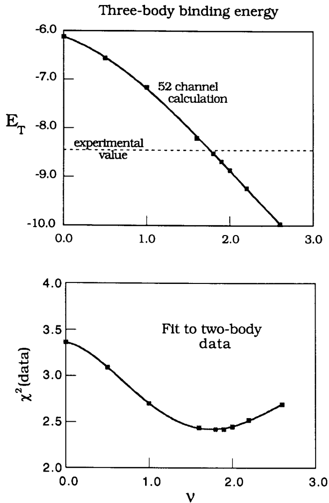
Figure 4. Triton binding energy, E_T (upper panel) and the \chi^2 for the fits to the two body data (lower panel) versus the scalar meson off-shell parameter \nu defined in the text. Note that the experimental binding energy and the best fits to the two body data are both obtained at about the same value of \nu \simeq 1.9 .
