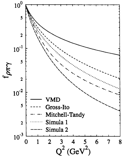
Figure 6: Various models of the \rho\pi\gamma form factor.
