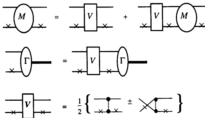
Figure 2: Diagrammatic representation of the spectator equations for NN scattering, the dNN vertex, and the OBE kernel.
