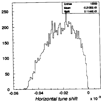
Fig.7. Horizontal tune shift distributions of the beam particles. For the same conditions as fig.6.
