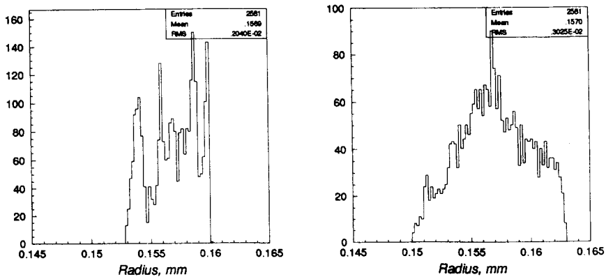
Fig.12. Distributions of the radial positions of the electron with incoming angle of 0^\circ (left) and 1^\circ (right).
