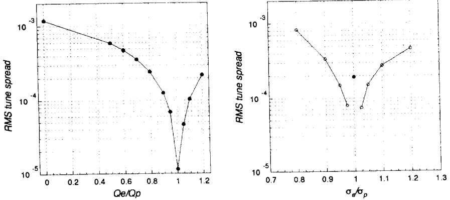
Fig.9. RMS tune spread of the beam particles : (left) versus the ratio of the electron to proton bunch charges. Displacement of the electron bunch is 0.1 \sigma . The leftmost point corresponds to the case without compensation. (right) versus the ratio of the rms size of the electron to proton bunch (white circles). Black circle presents the result for a cylindrical electron bunch (with radius r_e = 1.3\sigma_p and Q_e = 0.6Q_p ).
