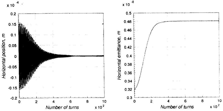
Fig.3. Oscillations of the beam centroid (left) and growth of the relative-to-centroid beam emittance (right) after an initial beam displacement of 1 \sigma . No compensation.
