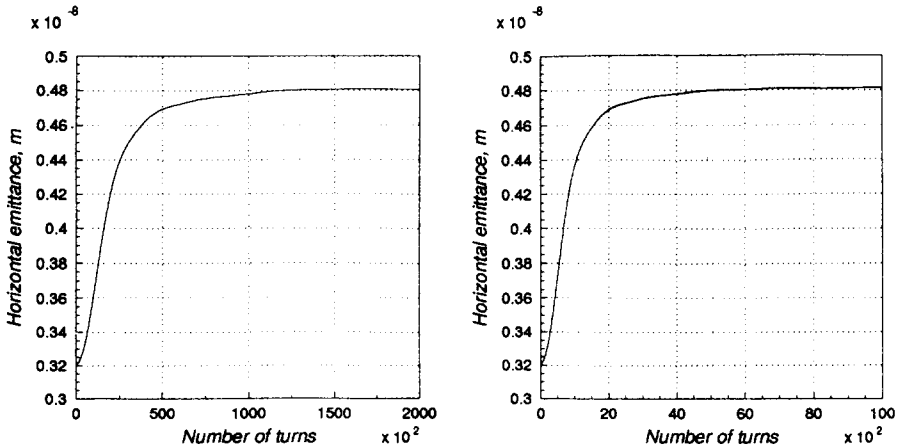
Fig.6. Growth of the relative-to-centroid beam emittance after an initial beam displacement of 1 \sigma . For the displacement of the compensating electron beam from the design orbit : 0.1 \sigma (left), 0.5 \sigma (right).
