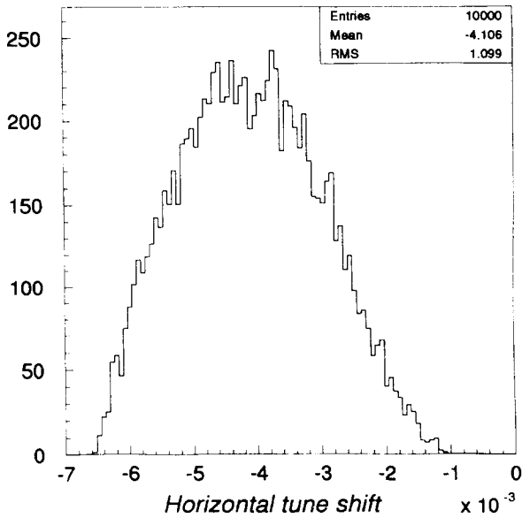
Fig.4. Horizontal tune shift distribution of the beam particles generated by the beam-beam interactions. No compensation.
