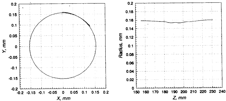
Fig.11. The trajectory of a 10 keV electron with an impact parameter of 160 \mu\text{m} inside a proton bunch when a solenoidal magnetic field of 2 T is applied: (left) X-Y view, (right) Z-R view (R is a distance of an electron from the center of a proton bunch).
