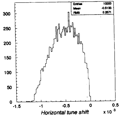
Fig.7. Horizontal tune shift distributions of the beam particles. For the same conditions as fig.6.
