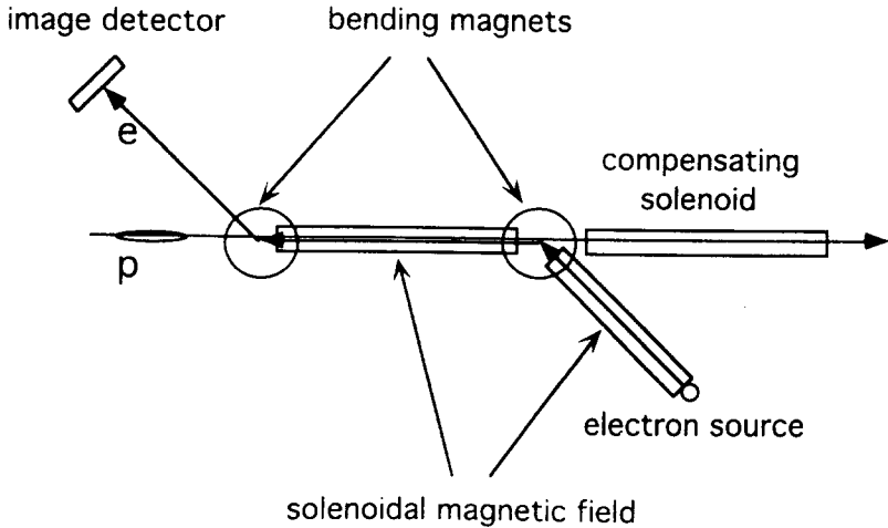
Fig.5. Scheme of the device for the beam-beam effect compensation. A low energy electron beam collides with a bunch of protons. The electron beam distribution is kept stable by a solenoidal magnetic field. After the collision the electron beam is deflected to the image detector which is used for steering the electron beam relative the proton bunch.
