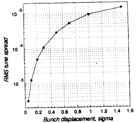
Fig.8. Decoherence time expressed in number of turns (left) and RMS tune spread of the beam particles (right) versus the electron beam displacement. The rightmost point corresponds to the case without compensation. The curve is drawn to guide the eye.
