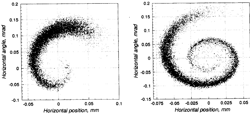
Fig.2. The distributions of the beam in phase space after 200 turns (left), 400 turns (right). Initial horizontal beam displacement is 3\sigma , where \sigma is the rms beam size.
