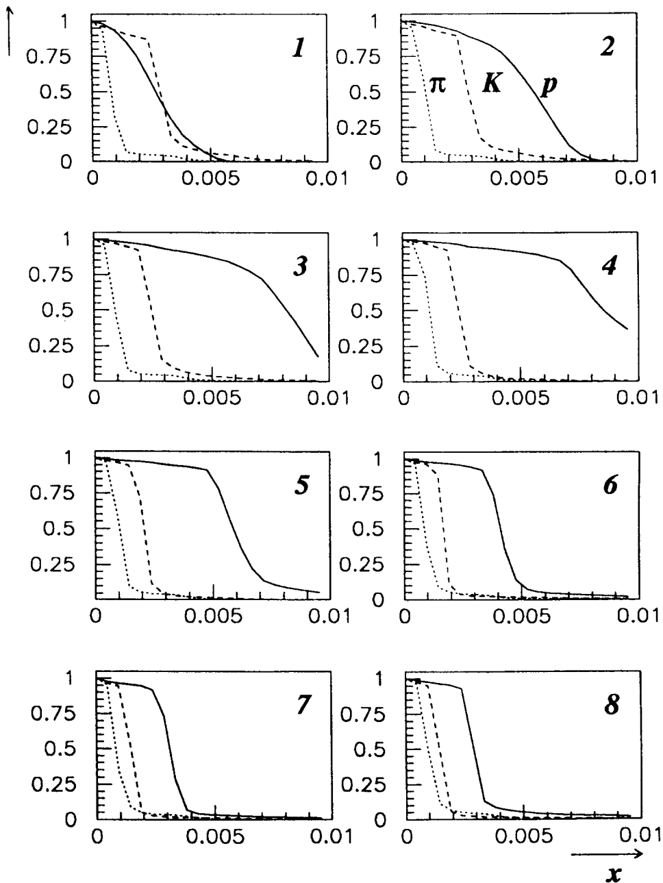
Fig.10. The \pi, K, p detection efficiencies in the BD hodoscope vs the x parameter defining the threshold.
