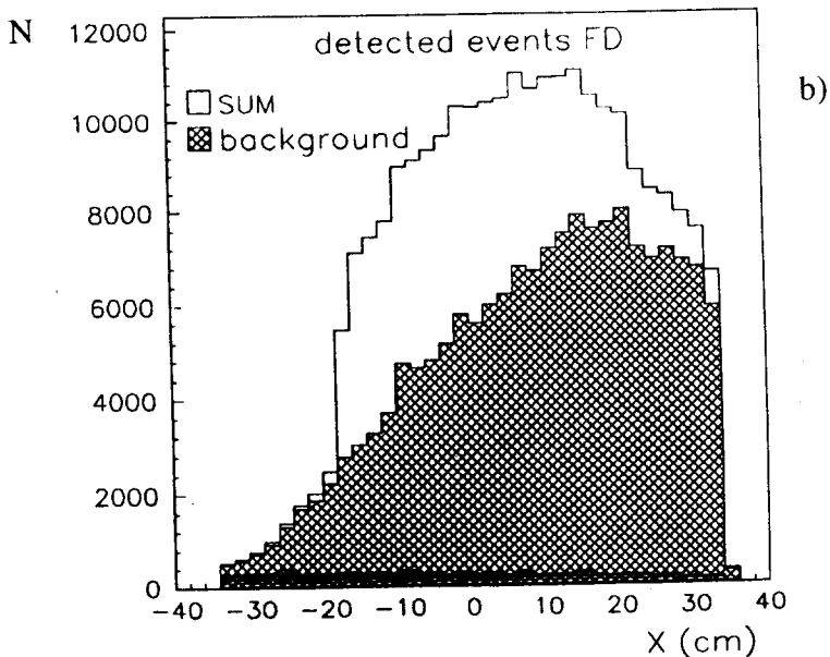
Fig.7. Distribution of all detected particles along the transverse axis of the BD(a) and FD(b) hodoscopes. The point x = 0 corresponds to the hodoscope center. The shaded area corresponds to the background events from reactions (1,2,3).
