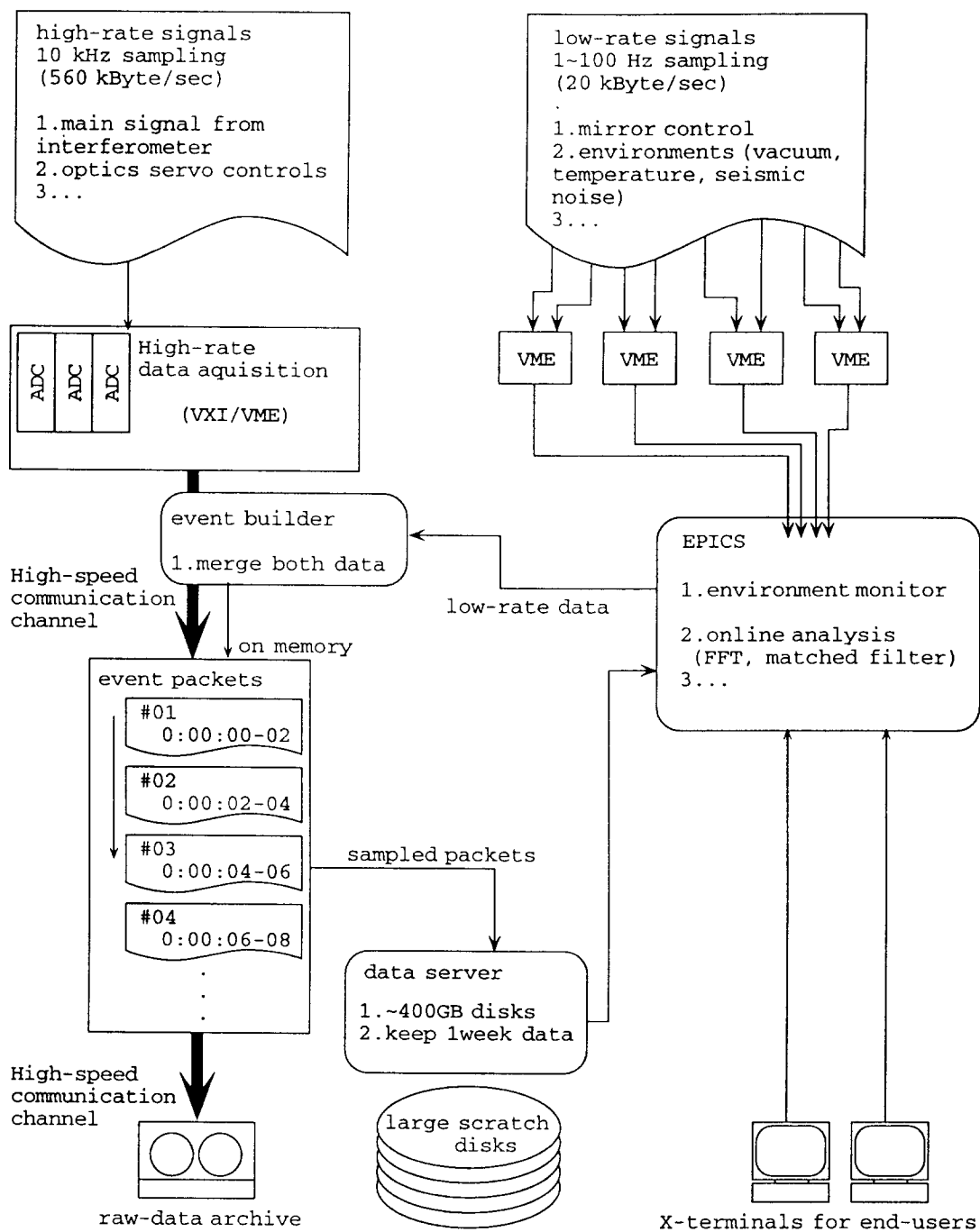
Figure 1: Schematic view of the data flows between the high-rate data-acquisition, the EPICS, the event builder, the data server, and the raw-data archiver.
