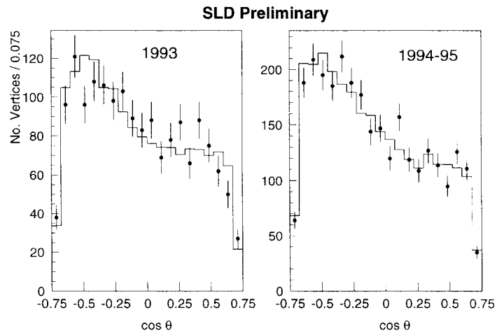
Figure 9: Distribution of B line of flight with respect to the positron beam, signed by the product of electron polarization and reconstructed charge for data (points) and Monte Carlo (histograms).
