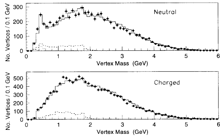
Figure 8: Mass of reconstructed secondary vertex for charged and neutral decays in the topological vertex analysis for data (points) and Monte Carlo (solid histograms). The dashed(dotted) histograms represent the charm( uds ) contribution from Monte Carlo.
