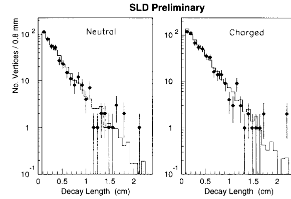
Figure 3: Decay length distributions for charged and neutral decays in the semileptonic analysis for data (points) and Monte Carlo corresponding to the best fit (histograms).
