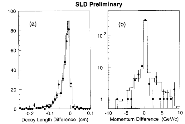
Figure 11: Distributions of the differences (semileptonic - topological) between reconstructed decay lengths and between momenta in the semileptonic and topological analyses for data (points) and Monte Carlo (histograms).
