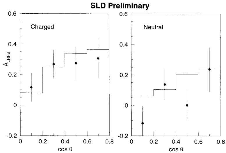
Figure 2: The Left-Right Forward-Backward asymmetry for charged and neutral decays in the semileptonic analysis for data (points) and Monte Carlo (histograms).
