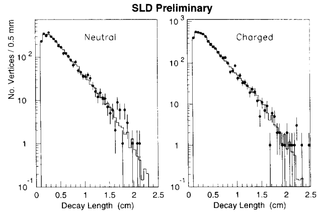
Figure 10: Decay length distributions for neutral and charged decays in the topological analysis for data (points) and Monte Carlo corresponding to the best fit (histograms).
