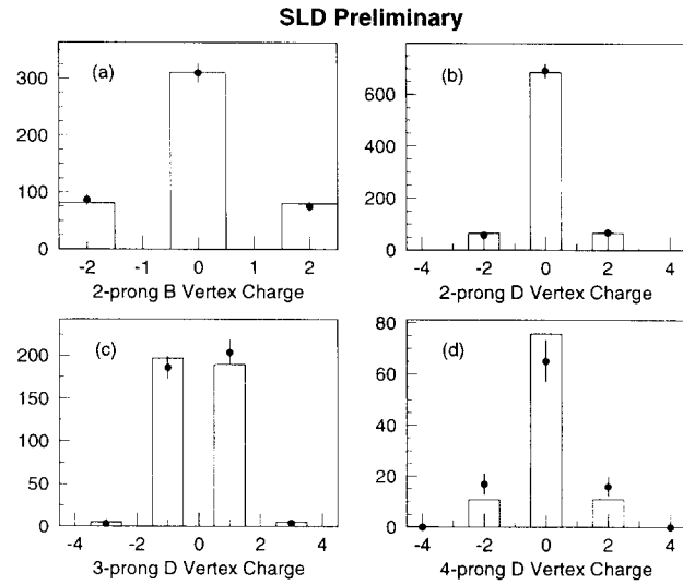
Figure 1: Comparison of charge assignment between the data (points) and Monte Carlo (histograms) for the semileptonic analysis.
