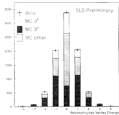
Figure 7: Distribution of charges reconstructed by the topological analysis for data (points) and Monte Carlo (histogram).
