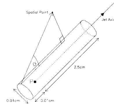
Figure 4: Construction of \alpha , the angular displacement.
