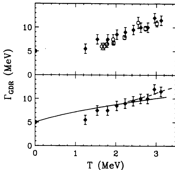
Figure 3. The widths of the GDR from the 50 MeV/nucleon inelastic scattering reaction (diamonds) compared to previous inclusive fusion measurements in ^{108-112}\text{Sn} nuclei (top) and adiabatic coupling calculations performed by Ormand et al. [18] (bottom). The fusion data were taken from Ref. [1] (o) and Ref. [2] (□).
