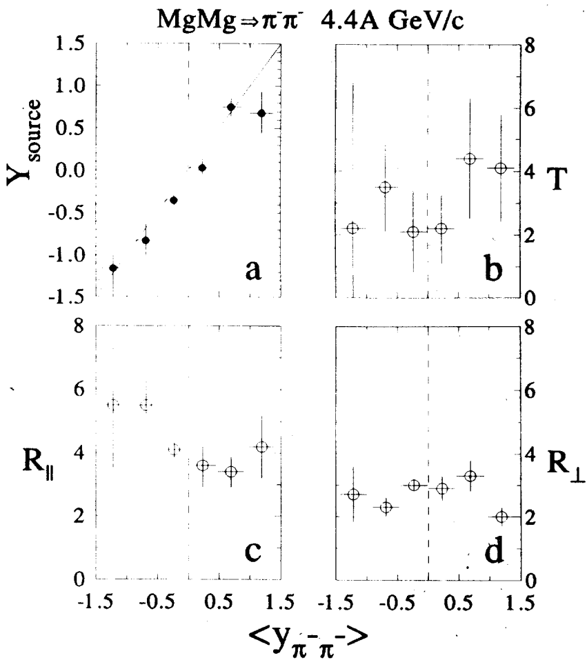
Fig.1 a): The rapidities of different elements of the production volume emitting \pi^- pairs having different mean rapidities. Straight line is Y_{\text{source}} = \langle y_{\pi^- \pi^-} \rangle . b),c),d): Root-mean-square dispersion of \pi^- emission times and root-mean-square radii of the production volume elements in their rest frames. The horizontal bars designate the bounds of pair mean rapidity intervals.
