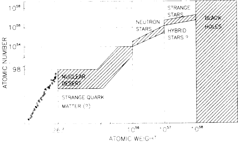
Figure 1: The overall chart of nucleides
