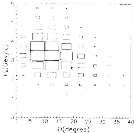
Figure 7. The expected angular and momentum distributions of H dihyperons formed within a fireball with T_H = 150 \text{ MeV} in central Mg-Mg collisions: the black circle – detected event.
