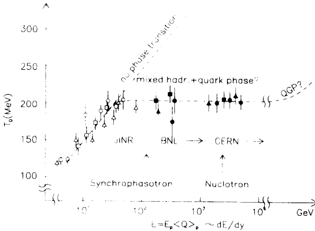
Figure 6. Inverse slope parameter of invariant cross section T_0 versus E = E_P \cdot Q , where Q - number of nucleon-participants ( degree of centrality ); open circles, triangles, squares - K^0 , \Lambda , proton data of JINR; black circles, triangles, squares - K , \Lambda and proton data of BNL 12 and CERN 13 .
