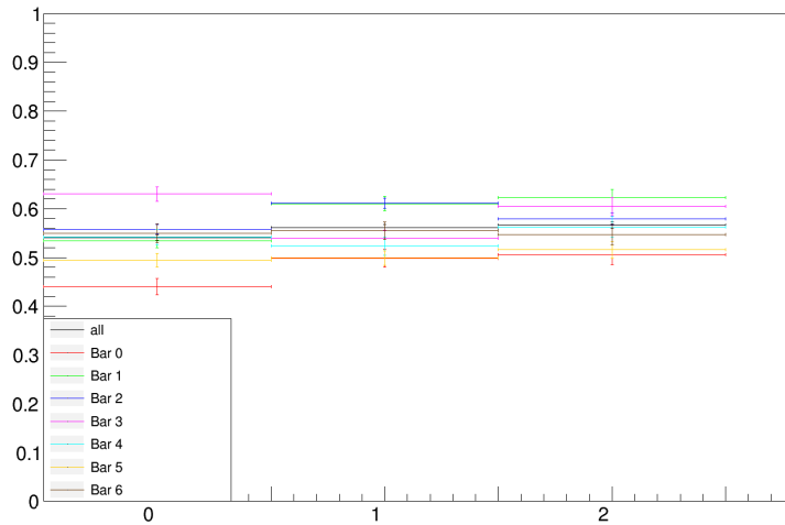
Figure 6. Relative hit rate of the Veto 3 as a function of the hit position. Each bin is the average of 12 cm. Bin 0 is the side furthest from the readout SiPM. Bin 1 is the central region. The last group is closest to the readout side.
