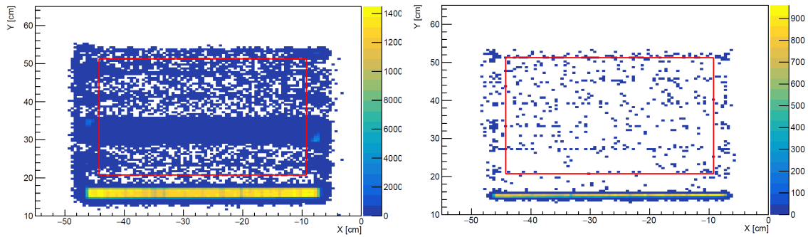
Figure 2. The extrapolated position of the reconstructed Scifi track at Veto plane 1 (left) and Veto plane 2 (right). The red square encloses the fiducial area which was used for the observation of neutrino interactions [2].
