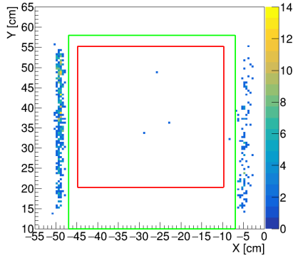
Figure 12. The extrapolated position of the reconstructed SciFi tracks at Veto 1 for events without any fired Veto channel in all three planes. The red square encloses the fiducial area used for the 2022-2023 analyses, while the green rectangle represents the fiducial area used in the 2024 Veto inefficiency study.
