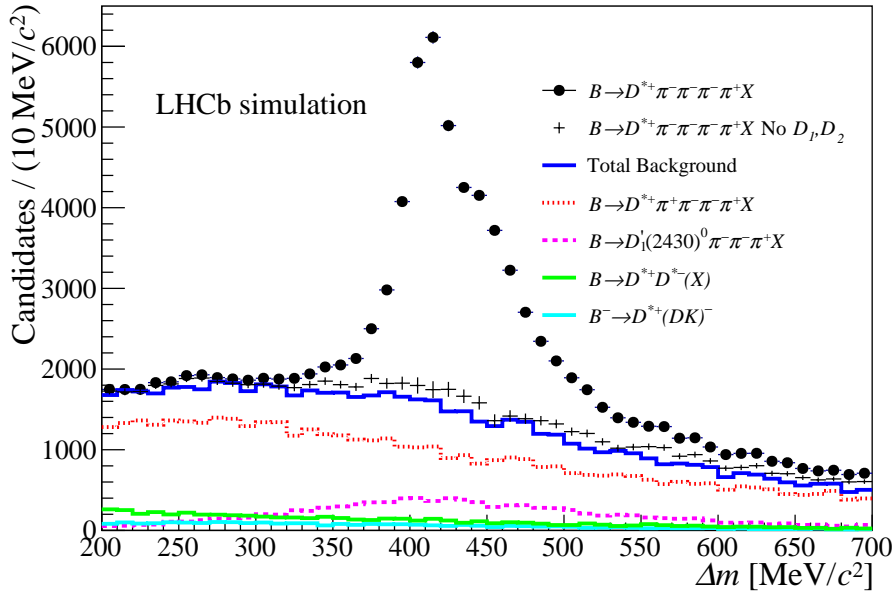
Figure 5: Distribution of the \Delta m mass difference for all selected D^{*+} candidates in the inclusive simulated sample (black circles) compared to the WS sample extracted from the same dataset. The background under the \Delta m peak in RS sample (black crosses) corresponds to RS simulated events not containing a D_1(2420)^0 or D_2^*(2460)^0 meson. A good agreement is found between this component and the (dark blue) total background estimate which is the sum of the WS candidates plus RS candidates containing either a D_1'(2400)^0 meson, a D^{*+}D^{*-} pair, or three-body D^{*+}(DK)^- in the final state.
