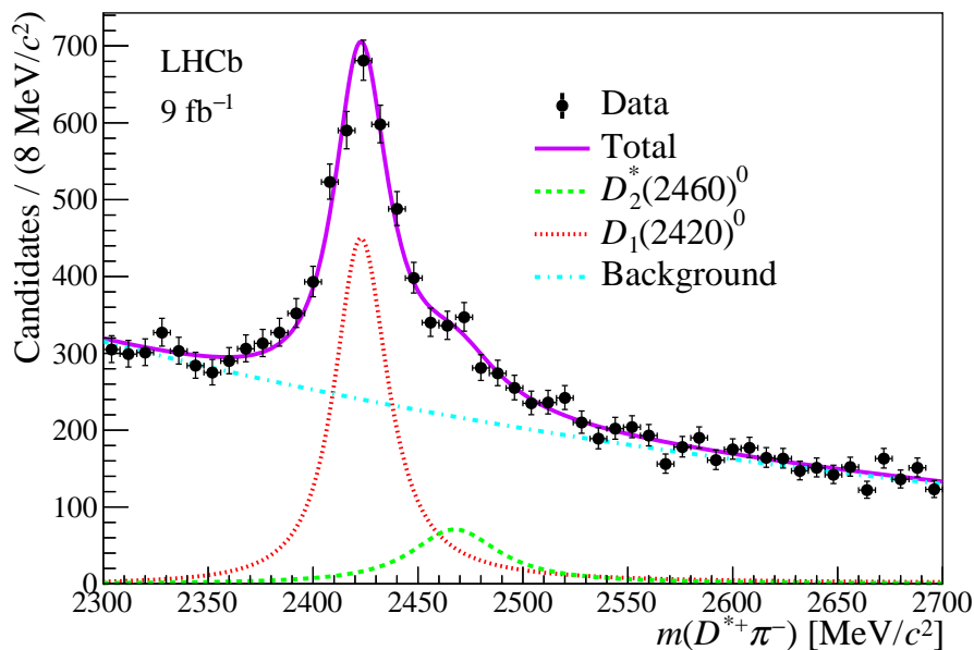
Figure 1: Distribution of the D^{*+}\pi^- mass for all selected D^{**0}\pi^-\pi^-\pi^+ candidates in the full dataset, with the result of the fit also shown. A potential D_1'(2400)^0 component can not be distinguished from the background.
