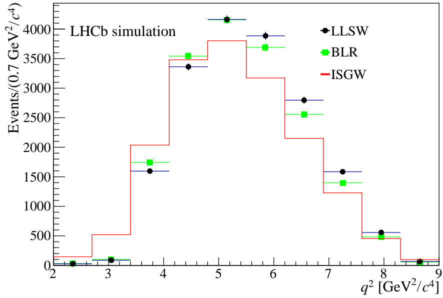
Figure 6: Distribution of the q^2 observable for simulated B^- \rightarrow D_1(2420)^0 \tau^- \bar{\nu}_\tau decays corresponding to the BLR [35], LLSW [34] and ISGW2 [33] form-factor models.
