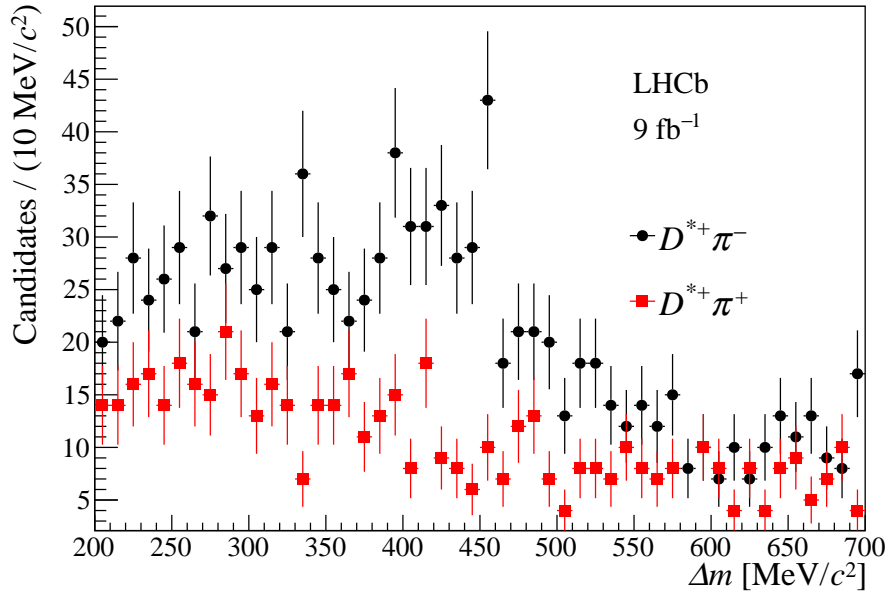
Figure 4: Distribution of the \Delta m mass difference for B \rightarrow (D^{*+}\pi^-)\bar{D}^0 candidates, with \bar{D}^0 reconstructed in the K^+\pi^-\pi^-\pi^+ final state.
