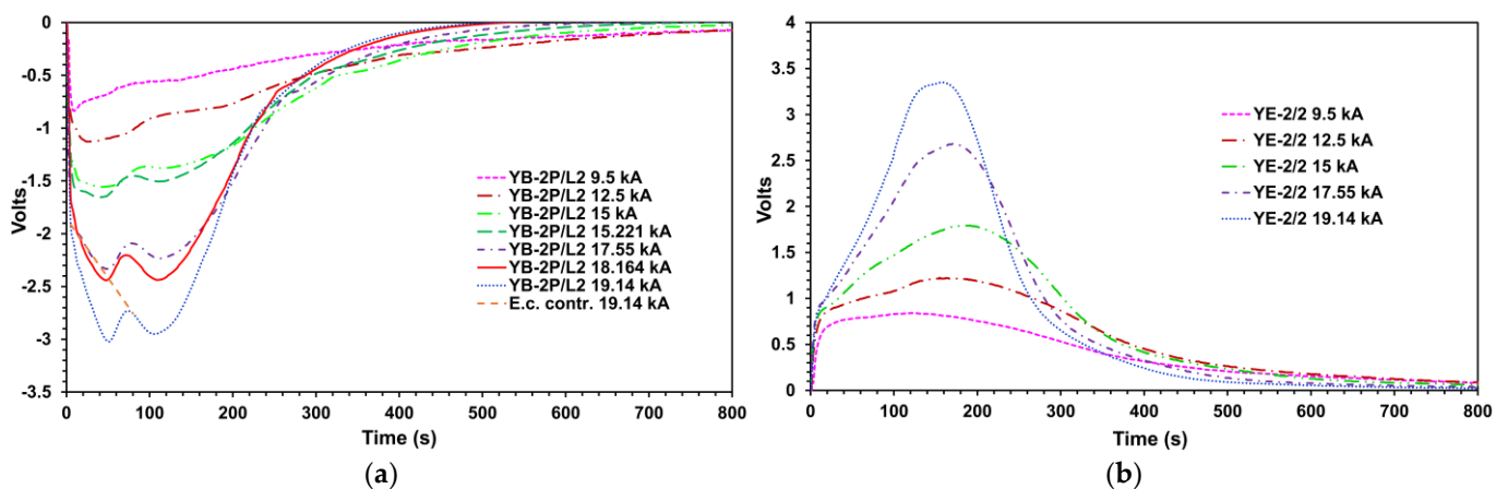
Figure 5. (a) Voltages measured in the flux loop P on the L2 layer of the external barrel wheel YB-2 during all seven fast discharges performed with different initial magnet currents. The orange short-dashed line cuts the contribution of the eddy currents to the signal at the beginning of the magnet fast discharge performed from the current of 19.14 kA. This contribution has been estimated [6] at the level of 4.6% into the integrated magnetic flux. (b) Voltages measured in the middle flux loop 2 of the endcap disk YE-2 during five fast discharges performed from different magnet currents.
