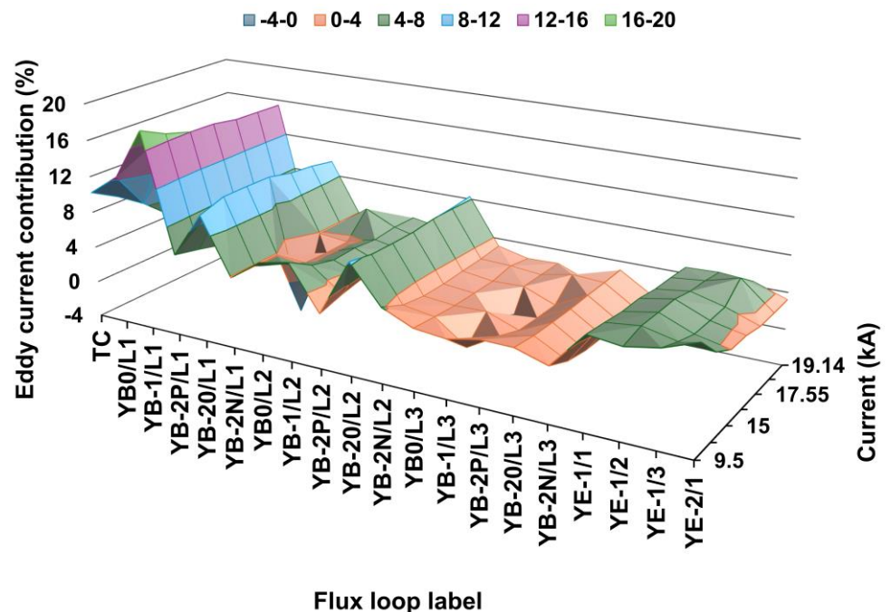
Figure 7. The eddy current contributions to 20 flux loops vs. initial currents of the fast discharges.
