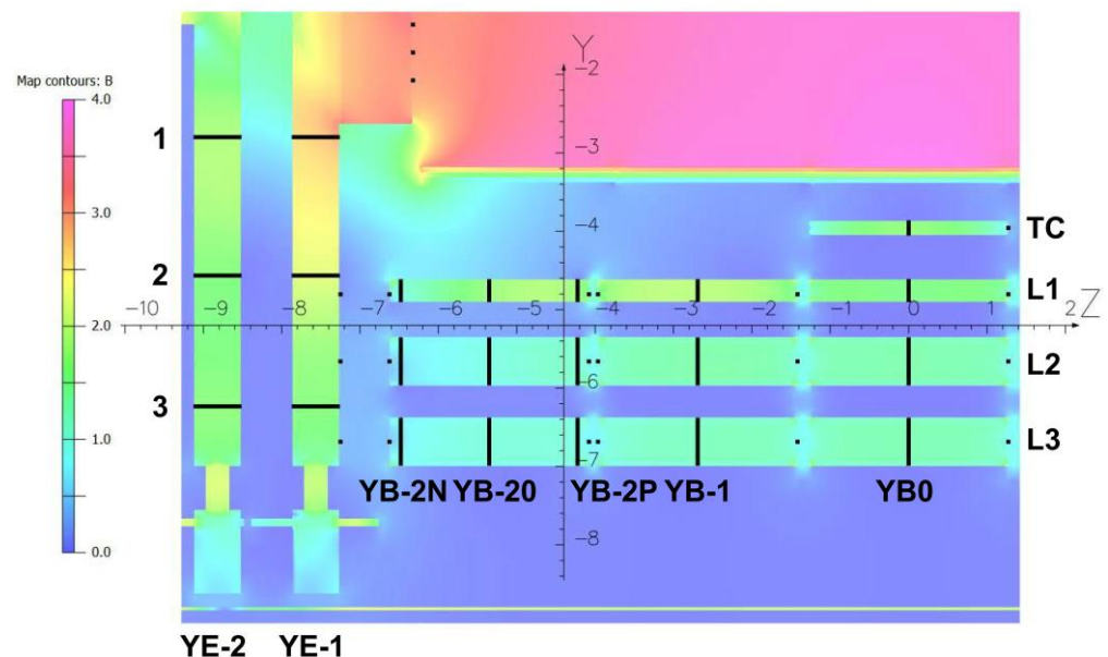
Figure 1. Modeled distribution of the magnetic flux density B in Tesla in the vertical YZ -plane of the flux loop location area. Sixteen flux loops are installed in the 30° azimuthal sector at 270° of the CMS magnet barrel flux-return yoke on four layers (TC, L1, L2, L3) of the central barrel wheel YB0, and on three layers (L1, L2, L3) of the barrel wheels YB-1 and YB-2 at negative Z -coordinates, shown in meters on the Z -axis. Six flux loops are wound at the distances 1, 2, and 3 along the 18° azimuthal sector at 270° of the CMS endcap thick disks YE-1 and YE-2 [6]. The black lines indicate the Y- or Z-positions of the loop cross-sections. The small black squares indicate the projections to the YZ -plane of the 3D B-sensor locations installed on the surfaces of the yoke steel blocks.
