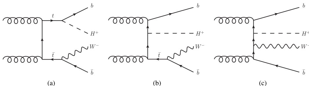
Figure 1: Examples of leading-order Feynman diagrams contributing to the production of charged Higgs bosons in pp collisions: (a) double-resonant top-quark production that dominates at low H^+ masses, (b) single-resonant top-quark production that dominates at large H^+ masses, (c) top-quark exchange production. The interference between these three main diagrams becomes most relevant in the intermediate-mass region.
