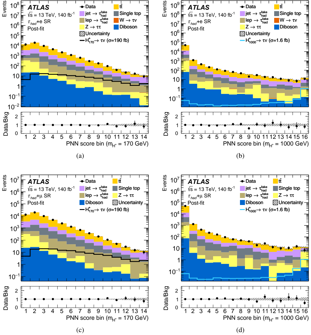
Figure 6: PNN score distributions after the fit to data (“Post-fit”) under the background-only hypothesis in the SR of the \tau_{\text{had}}+\text{electron} sub-channel for the (a) 170 GeV and (b) 1000 GeV m_{H^+} hypotheses and \tau_{\text{had}}+\text{muon} sub-channel for the (c) 170 GeV and (d) 1000 GeV m_{H^+} hypotheses. The signal distribution of the 170 GeV (1000 GeV) H^+ mass hypothesis is shown by the solid black (teal) line, where the signal distribution is scaled to its expected 95% CL limit. The lower panel of each plot shows the ratio of data to the SM background prediction. The uncertainty bands include all statistical and systematic uncertainties. Bin boundaries are optimized for the best sensitivity of the final fit (see Section 5) but are displayed as equidistant for better readability.
