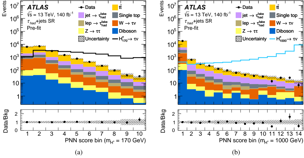
Figure 3: PNN score distributions before the fit to data (“Pre-fit”) in the SR of the \tau_{\text{had}}+\text{jets} for the (a) 170 GeV and (b) 1000 GeV m_{H^+} hypotheses. The lower panel of each plot shows the ratio of data to the SM background prediction. The uncertainty bands include all statistical and systematic uncertainties. Bin boundaries are optimized for the best sensitivity of the final fit (see Section 5) but are displayed as equidistant for better readability. Also shown are the expected signal distributions normalized to the total background yield.
