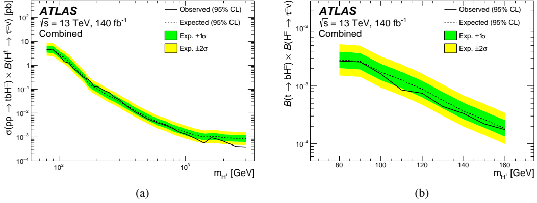
Figure 7: Observed and expected 95% CL exclusion limits on (a) \sigma(pp \rightarrow tbH^+) \times \mathcal{B}(H^+ \rightarrow \tau\nu) and (b) \mathcal{B}(t \rightarrow bH^+) \times \mathcal{B}(H^+ \rightarrow \tau\nu) as a function of m_{H^+} , from a combined fit in the \tau_{\text{had-vis}} + \text{jets} and \tau_{\text{had-vis}} + \text{lepton} channels. The surrounding shaded bands correspond to the 1\sigma and 2\sigma confidence intervals around the expected limit.
