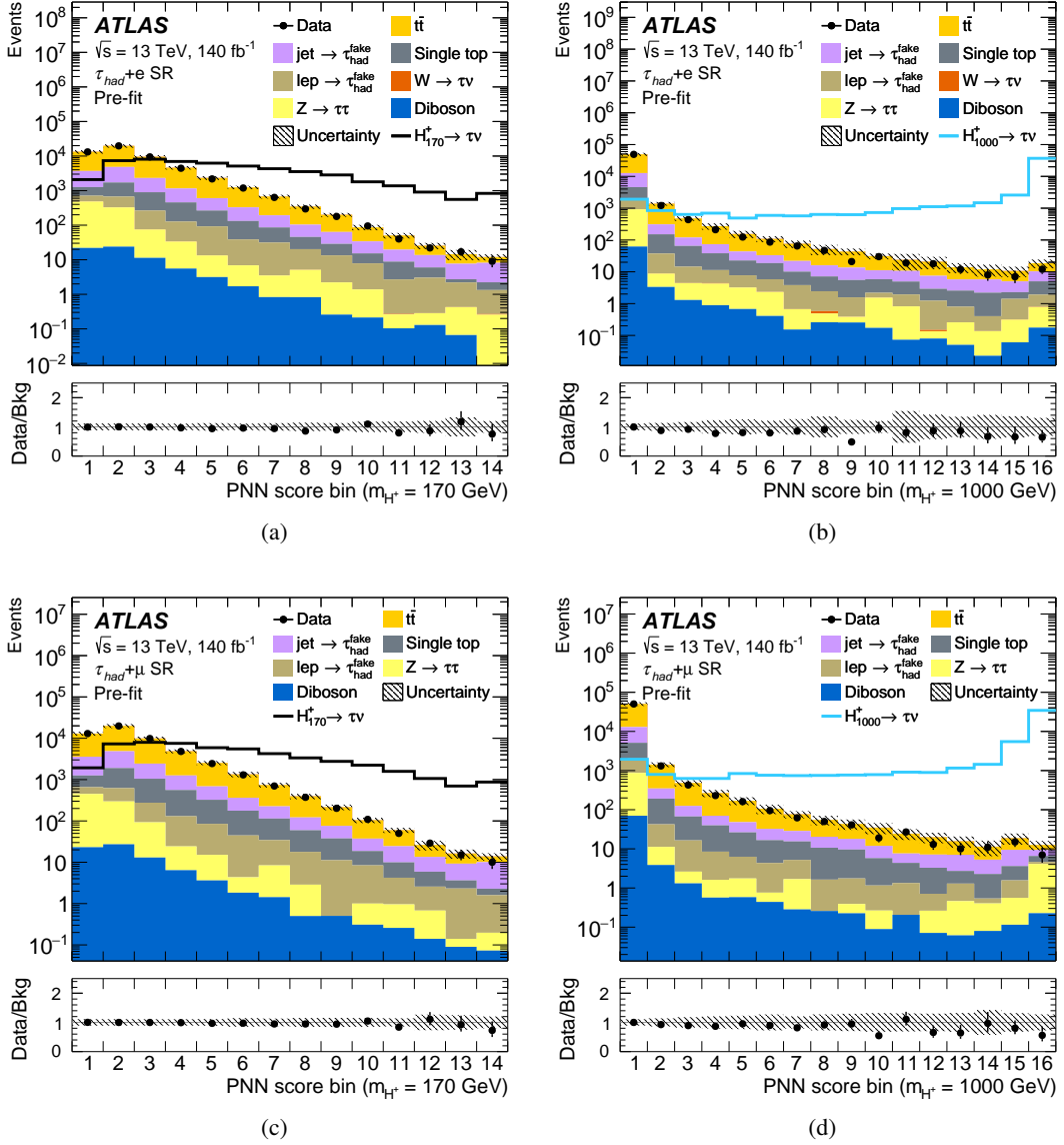
Figure 4: PNN score distributions before the fit to data (“Pre-fit”) in the SR of the \tau_{\text{had}}+\text{electron} sub-channel for the (a) 170 GeV and (b) 1000 GeV m_{H^+} hypotheses and \tau_{\text{had}}+\text{muon} sub-channel for the (c) 170 GeV and (d) 1000 GeV m_{H^+} hypotheses. The lower panel of each plot shows the ratio of data to the SM background prediction. The uncertainty bands include all statistical and systematic uncertainties. Bin boundaries are optimized for the best sensitivity of the final fit (see Section 5) but are displayed as equidistant for better readability. Also shown are the expected signal distributions normalized to the total background yield.
