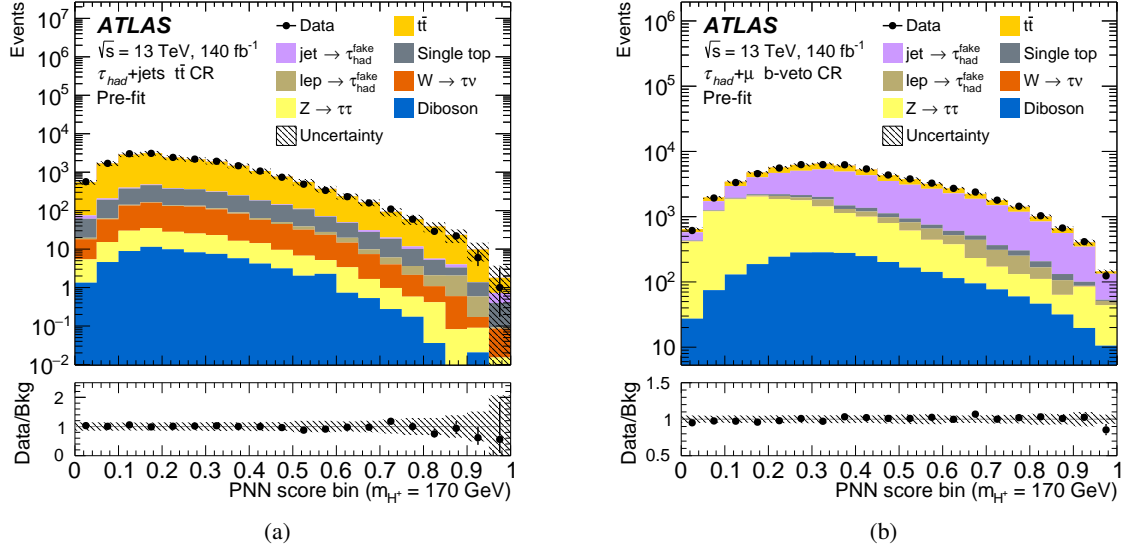
Figure 2: Predicted and measured PNN score distributions before the fit to data (“Pre-fit”) in (a) the t\bar{t} enriched CR of the \tau_{\text{had}}+\text{jets} channel and (b) the b -veto CR of the \tau_{\text{had}}+\mu channel enriched in the W/Z+\text{jets} events with jets faking \tau_{\text{had-vis}} , for the 170 GeV m_{H^+} hypothesis. The lower panel of each plot shows the ratio of data to the SM background prediction. The uncertainty bands include all statistical and systematic uncertainties. The bin boundaries of these distributions are spaced equally at intervals of 0.05 and do not represent the binning scheme used in the final fits.
