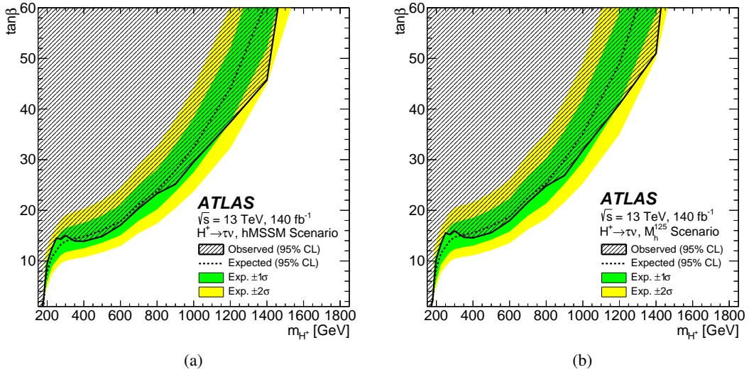
Figure 8: Observed and expected 95% CL exclusion limits on \tan\beta as a function of m_{H^+} , shown in the context of (a) the hMSSM and the (b) the M_h^{125} scenario of the MSSM, for m_{H^+} > 150 GeV and (1 \leq \tan\beta \leq 60) . The surrounding shaded bands correspond to the 1\sigma and 2\sigma confidence intervals around the expected limit.
