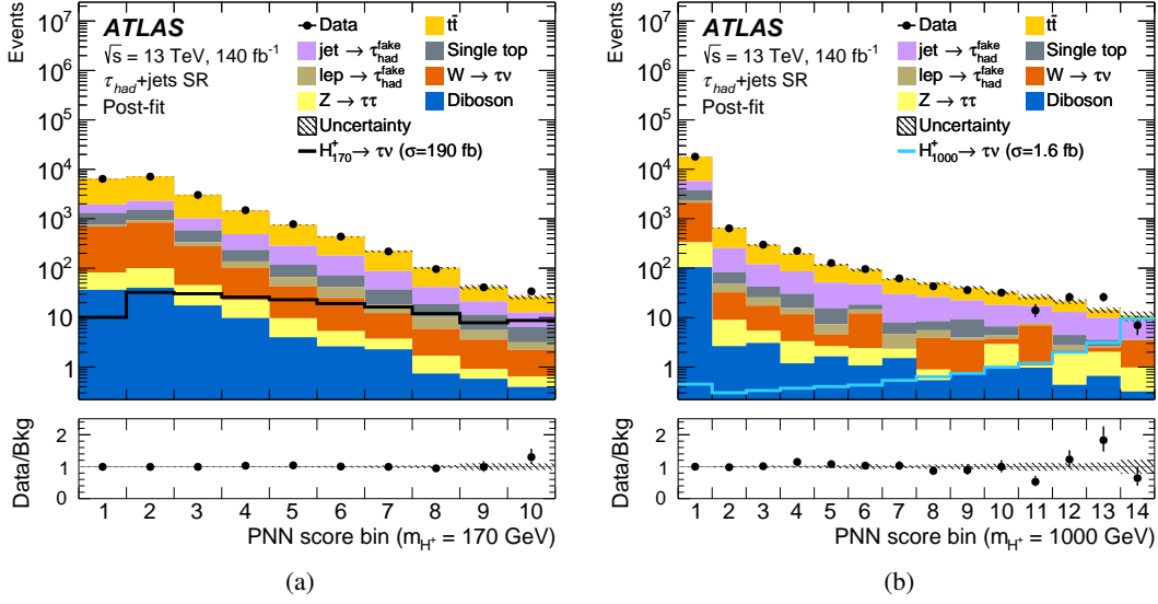
Figure 5: PNN score distributions after the fit to data (“Post-fit”) under the background-only hypothesis in the SR of the \tau_{\text{had}}+\text{jets} channel for the (a) 170 GeV and (b) 1000 GeV m_{H^+} hypotheses. The signal distribution of the 170 GeV (1000 GeV) H^+ mass hypothesis is shown by the solid black (teal) line, where the signal distribution is scaled to its expected 95% CL limit. The lower panel of each plot shows the ratio of data to the SM background prediction. The uncertainty bands include all statistical and systematic uncertainties. Bin boundaries are optimized for the best sensitivity of the final fit (see Section 5) but are displayed as equidistant for better readability.
