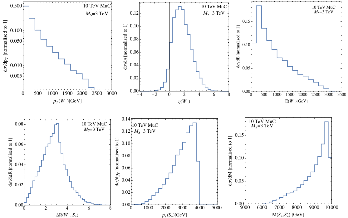
Figure 12. Kinematical distributions for the process \mu^- \mu^+ \rightarrow S_+ S_-^\dagger W^- evaluated at LO with MadGraph5_aMC, for a 10 TeV MuC and M_S = 3 TeV.
