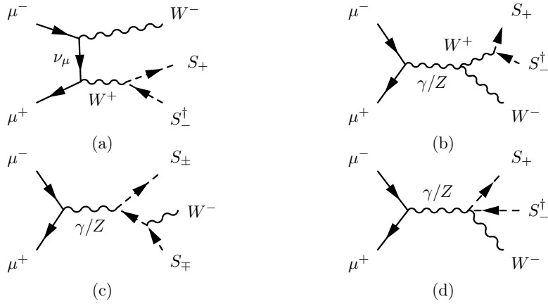
Figure 10. Leading-order Feynman diagrams for \mu^- \mu^+ \rightarrow S_+ S_-^\dagger W^- .
