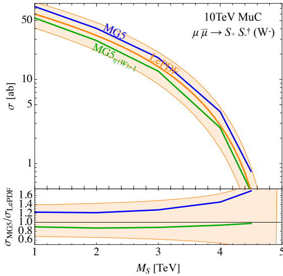
Figure 11. Cross section for the charged-current pair production of a heavy scalar doublet, at a 10 TeV MuC. Orange is the result obtained with LePDF (the band represents the scale uncertainty) with the muon neutrino PDF, blue and green are the MadGraph5_aMC results with no cuts and with a cut \eta(W) > 1 , respectively.
