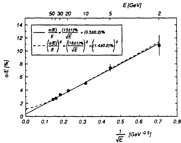
Fig. 2.5 Energy resolution of the semi-projective spaghetti calorimeter prototype as obtained in the X3 beam line in May. Preliminary results on tests performed on X5 in mid September confirm the above constant term with points taken up to 100 GeV. The scaling term seems to be smaller in the X5 tests indicating some energy spread problems in the X3 beam at low energy settings.
