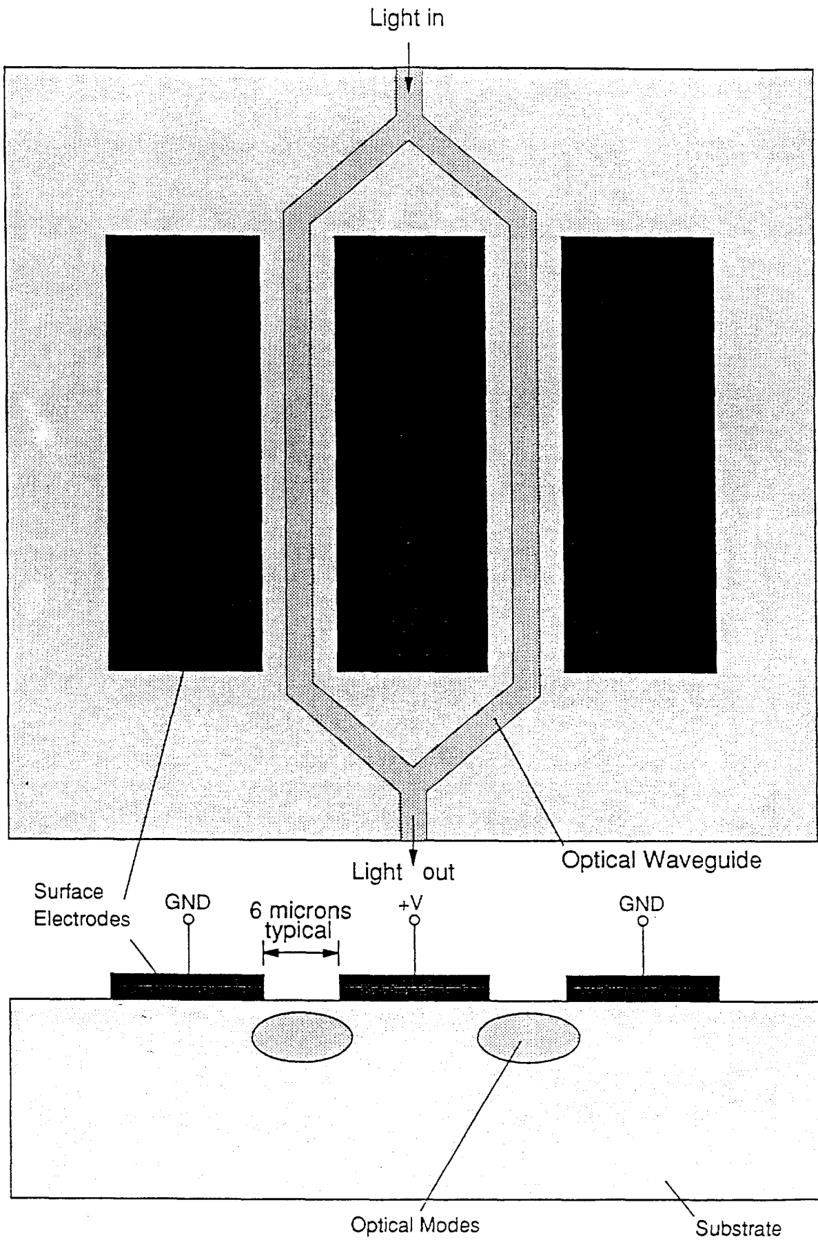
Fig. 1: Plan and Cross-Section of Electro-Optic Modulator
