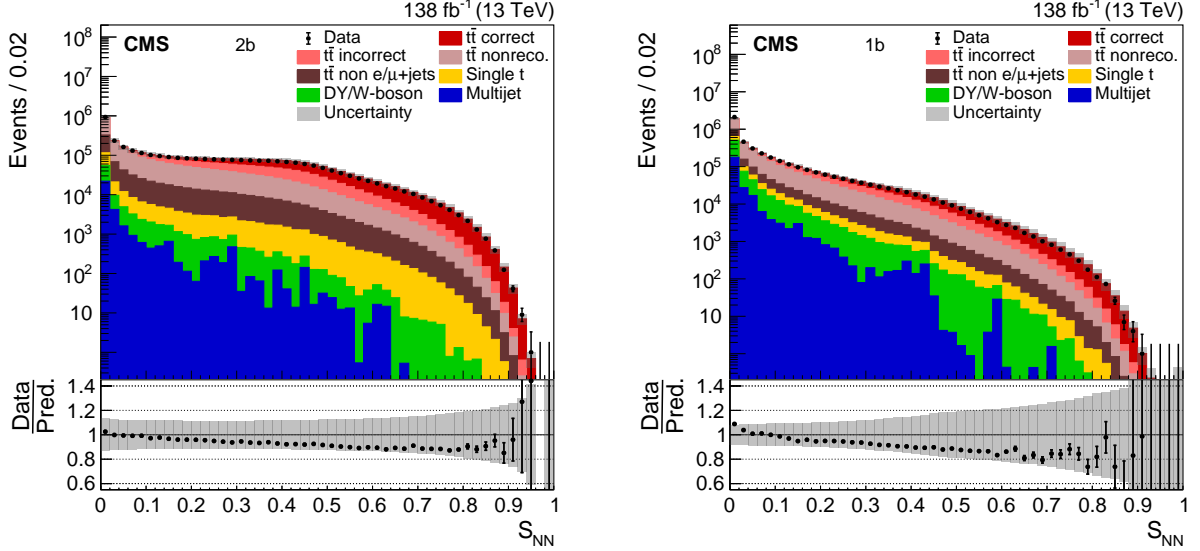
Figure 1: Distribution of S_{\text{NN}} in the 2b (left) and 1b (right) categories. The data (points) are compared to the prediction (stacked histograms). The t\bar{t} contribution is split into the correctly and incorrectly reconstructed, “nonreconstructable”, and non e/\mu +jets events. The gray uncertainty band indicates the combined statistical and systematic uncertainties in the prediction, while the vertical bars on the points show the statistical uncertainty of the data. The ratios of data to the predicted yields are provided in the lower panels.
