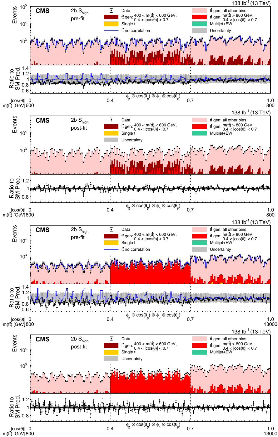
Figure 12: Pre- and post-fit distributions comparing the data (points) to the POWHEG+PYTHIA simulation (stacked histograms) for the full matrix measurement in bins of m(\bar{t}\bar{t}) vs. |\cos(\theta)| in the 2b S_{\text{high}} category. The x axis shows the bins of the unrolled 4-dimensional distribution of \phi_{\bar{p}}, \cos(\theta_{\bar{p}}), \phi_p, and \cos(\theta_p) , listed from the outermost to the innermost variable in each of the m(\bar{t}\bar{t}) vs. |\cos(\theta)| bins. The boundaries of the |\cos(\theta)| and m(\bar{t}\bar{t}) bins are labeled and indicated by dashed and solid lines, respectively. For the illustration of resolution effects, \bar{t}\bar{t} events generated in two selected m(\bar{t}\bar{t}) vs. |\cos(\theta)| bins are shown in different shades of red. All other \bar{t}\bar{t} contributions are shown in pink. A model without any polarization and spin correlation is shown as a blue line. The gray uncertainty band indicates the combined statistical and systematic uncertainties in the prediction. The vertical bars on the points show the statistical uncertainty. Ratios to the predicted yields are provided in the lower panels.
