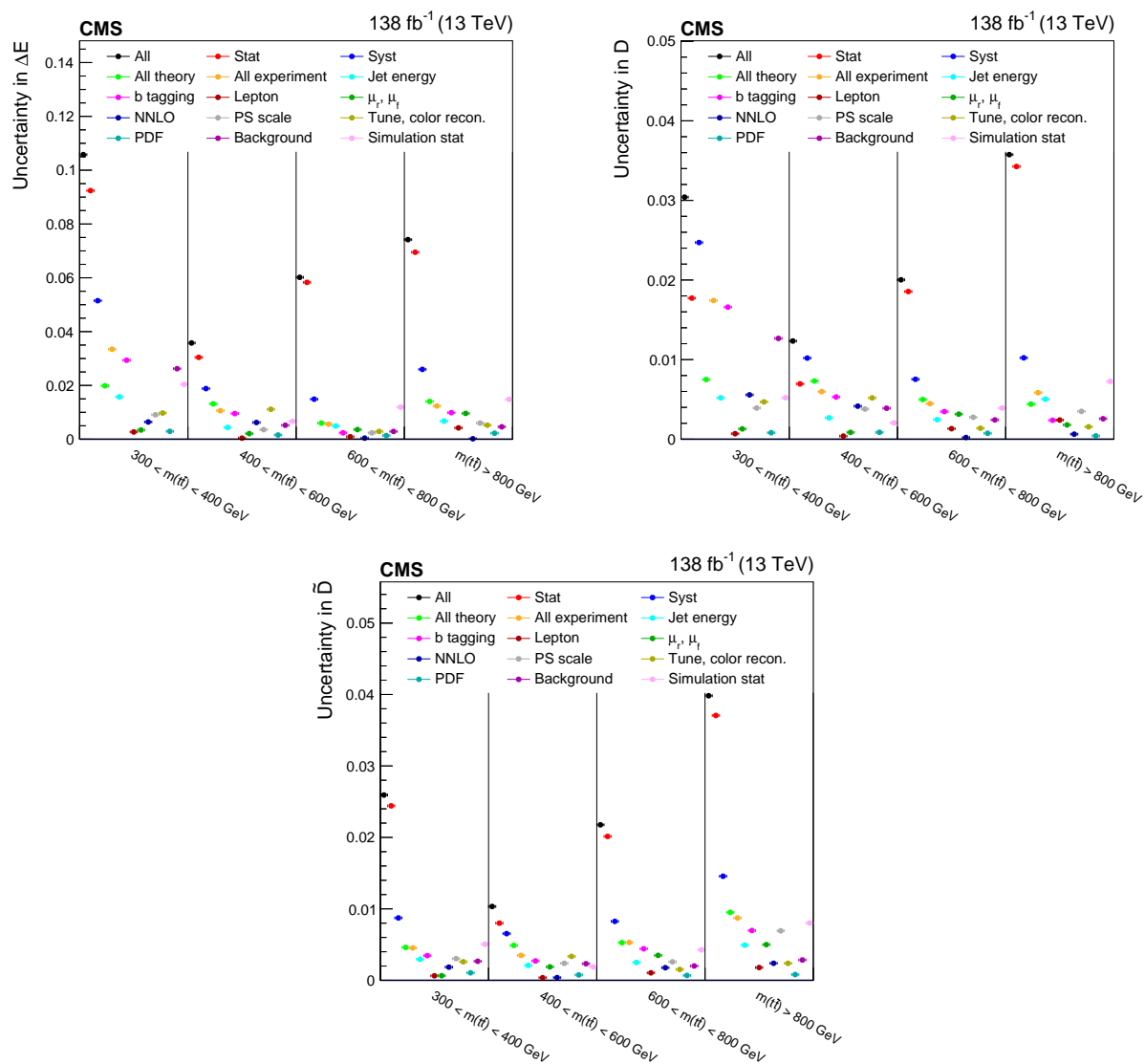
Figure 24: Contribution of individual uncertainty sources or groups of uncertainties in the measured \Delta_E , D , and \bar{D} in bins of m(\text{t}\bar{\text{t}}) .
