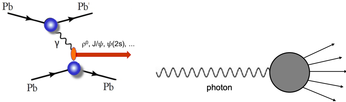
Figure 1 – Typical exclusive vector meson production in UPC (left). The photon can also break up the target (right).
