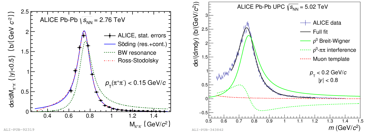
Figure 3 – a) Run 1 : \sim 7\text{k} events [19]. b) Run 2 : \sim 60\text{k} events [20].
