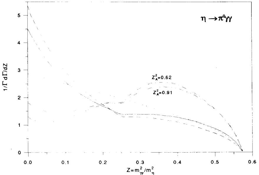
Fig. 2. Normalized differential decay probability for \eta \rightarrow \pi^0 \gamma \gamma as a function of Z = m_{\gamma\gamma}^2 / m_\eta^2 . The dotted line represents the phase space distribution. The dashed line corresponds to the calculation at O(p^6) without reduction of the resonances. The dash-dotted lines display the uncertainty in the reduction of meson resonances for different values of the parameter Z_A^2 . The solid line corresponds to the values of the coefficients L_i and d_i used in Ref. [11].
