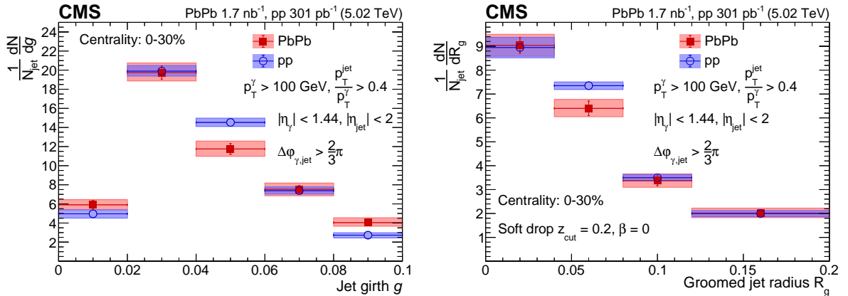
Figure 4: Unfolded distributions of jet girth g (left) and groomed jet radius R_g (right) of photon-tagged jets in PbPb and pp collisions for x_{\gamma j} \equiv p_T^{\text{jet}}/p_T^\gamma > 0.4 (selecting both more and less quenched jets). The bands represent the total uncertainties, whereas the vertical bars represent the statistical uncertainties.
