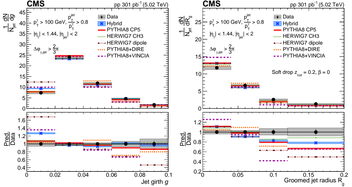
Figure 3: Unfolded distributions of jet girth g (left) and groomed jet radius R_g (right) of photon-tagged jets in pp collisions for x_{\gamma j} \equiv p_T^{\text{jet}}/p_T^{\gamma} > 0.8 . The upper panels show the comparison of the observable in pp collisions and predictions from simulated events. The lower panels show the corresponding ratios of the MC calculations and data. The bands represent the total experimental uncertainties, whereas the vertical bars represent the statistical uncertainties.
