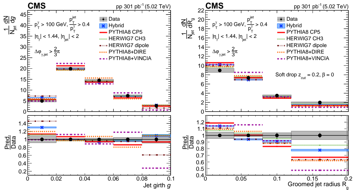
Figure 2: Unfolded distributions of jet girth g (left) and groomed jet radius R_g (right) of photon-tagged jets in pp collisions for x_{\gamma j} \equiv p_T^{\text{jet}}/p_T^{\gamma} > 0.4 . The upper panels show the comparison of the observable in pp collisions and predictions from simulated events. The lower panels show the corresponding ratios of the MC calculations and data. The bands represent the total uncertainties, whereas the vertical bars represent the statistical uncertainties.
