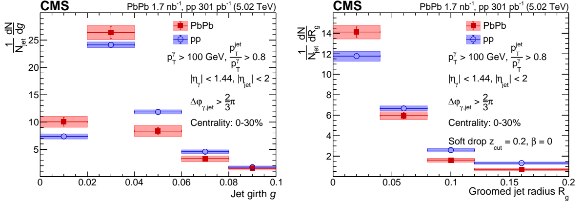
Figure 5: Unfolded distributions of jet girth g (left) and groomed jet radius R_g (right) of photon-tagged jets in PbPb and pp collisions for x_{\gamma j} \equiv p_T^{\text{jet}}/p_T^\gamma > 0.8 (selecting less quenched jets). The bands represent the total uncertainties, whereas the vertical bars represent the statistical uncertainties.
