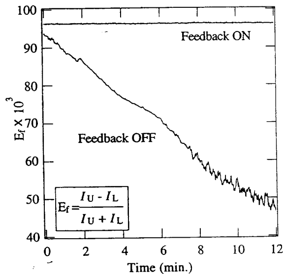
Fig. 4. Plot of Error Function vs. Time Illustrating Feedback Operation
