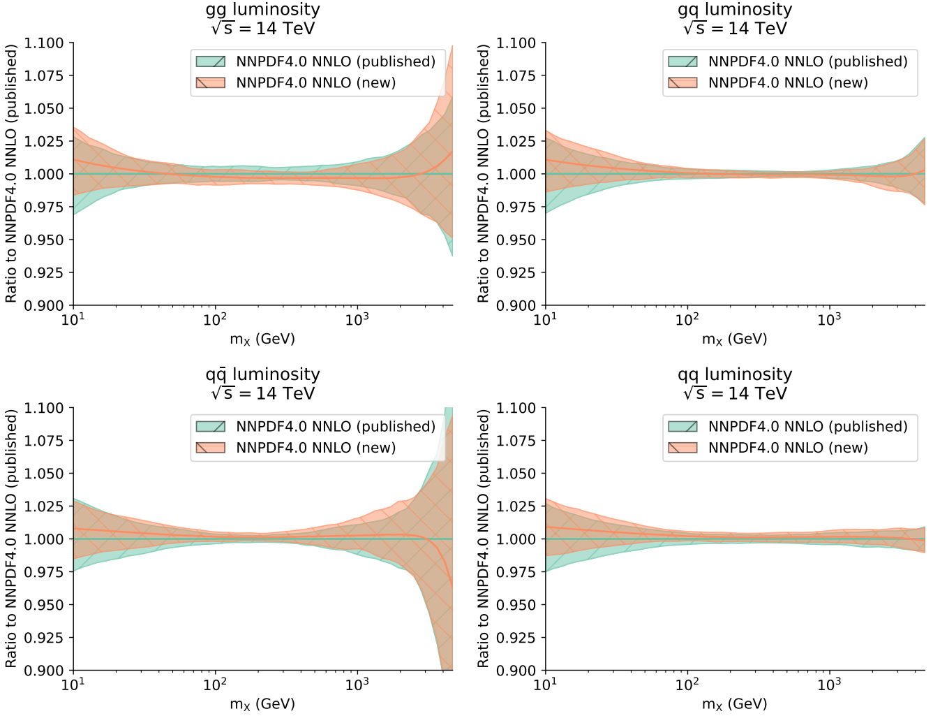
Figure A.5. Same as in Fig. A.4 at NNLO.
