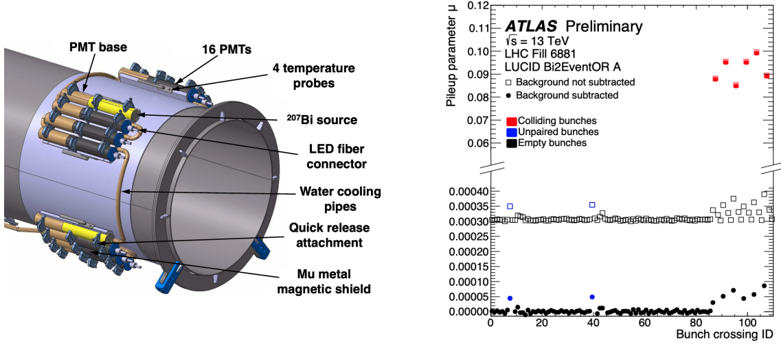
Figure 1: Left: Drawing of the LUCID-2 detector [5]. Right: Run averaged pileup parameter \mu as a function of the bunch-crossing identifier (BCID) as measured by the LUCID Bi2EventOR A algorithm. The empty squares (full circles) refer to the data before (after) ^{207}\text{Bi} background subtraction. The red markers refer to the colliding bunch slots, the blue ones to unpaired-bunch slots, and the black ones to nominally empty slots [7].
