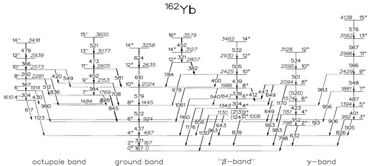
Figure 2. Low-lying levels of ^{162}\text{Yb} , from the in-beam work of [Md18] and the decay work of [Mc04], including the ground, “ \beta ”, \gamma -bands and octupole vibrational bands. Transitions in parenthesis have not been observed.
