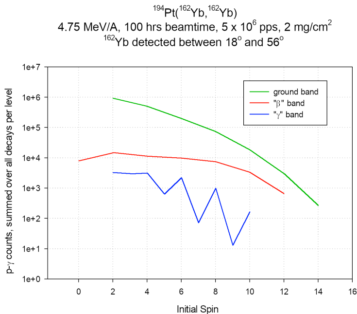
Figure. 3. Integrated p - \gamma coincidence counts of a safe Coulomb Excitation measurement for the levels of the ground, 0_2^+ and \gamma -bands of ^{162}\text{Yb} . The detected particle is ^{162}\text{Yb} .
