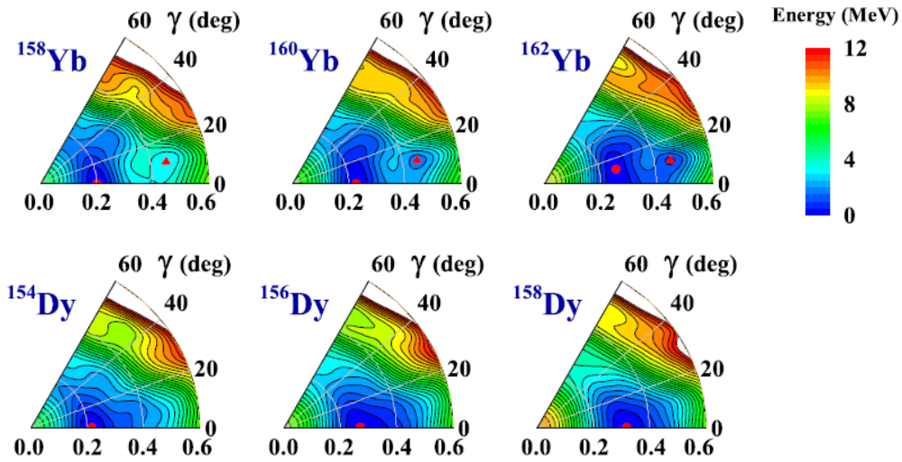
Figure 2. PES's of N=88 , N=90 and N=92 Dy and Yb isotones in the \beta - \gamma -plane. Minima are marked with red symbols, circles and triangles represent the global and secondary minima, respectively. The energy spacing in the contour lines is 0.25 MeV [Ma19]. RMF PES around N=90 [Ma19].
