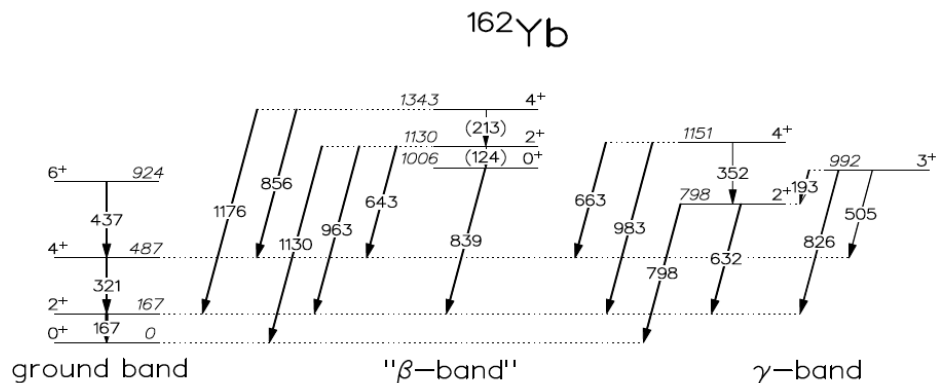
Figure 4. Close-up of the levels and related transitions of the ground, “ \beta ” and \gamma -bands of ^{162}\text{Yb} , as observed in \beta -decay [Mc04]. Transitions in parenthesis have not been observed.
