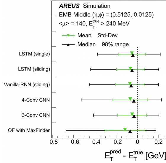
Figure 2: Reconstruction performance of the optimal filtering method and the various ML algorithms studied[4].
