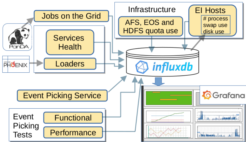
Figure 2: Functional schema for the monitoring system of the EventIndex components. Several modules collect information from multiple sources about the status of EventIndex processes (top left), functional and performance tests (bottom left) and the computing infrastructure (top right) and store this information in an InfluxDB database; the data are then displayed in Grafana dashboards.
