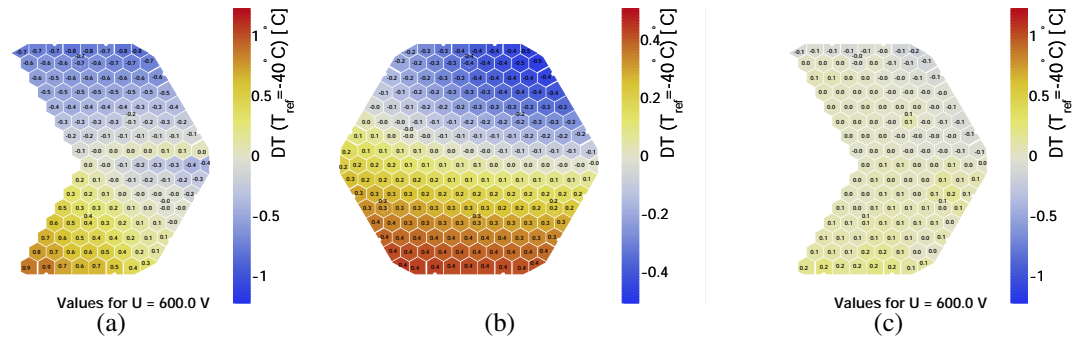
Figure 14: (a) Temperature differences derived from per-pad leakage currents between symmetric locations of a representative neutron-irradiated CE silicon sensors on the cold chuck at CERN. (b) Determined profile of temperature differences, modelled as a two-dimensional gaussian, across the sensor surface. (c) Closure check: derived temperature differences after accordingly correcting the measured per-pad leakage currents.
