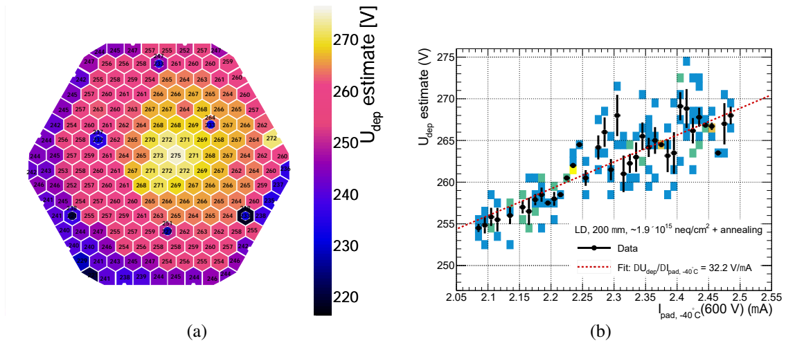
Figure 12: (a) Per-pad depletion voltage estimates for a 200 μm LD example sensor irradiated to 1.9 \times 10^{15} neq/cm 2 , and (b) their correlation to the per-pad leakage current, used as proxy for the delivered fluence.
