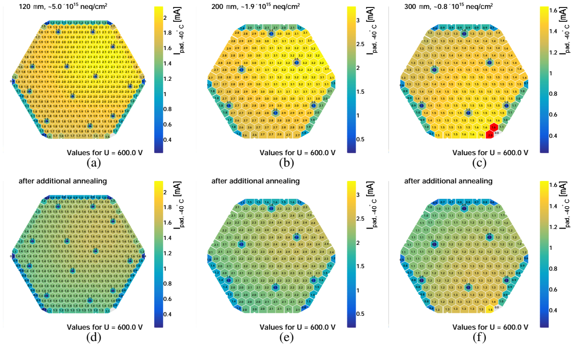
Figure 9: Per-pad leakage currents interpolated to an effective bias voltage of 600 V for three representative sensors from different irradiation rounds before (a-c) and after additional annealing (d-f). Red- or white-colored edge pads correspond to well-understood measurement effects, e.g. insufficient contact between the pogo pins and the pads.
