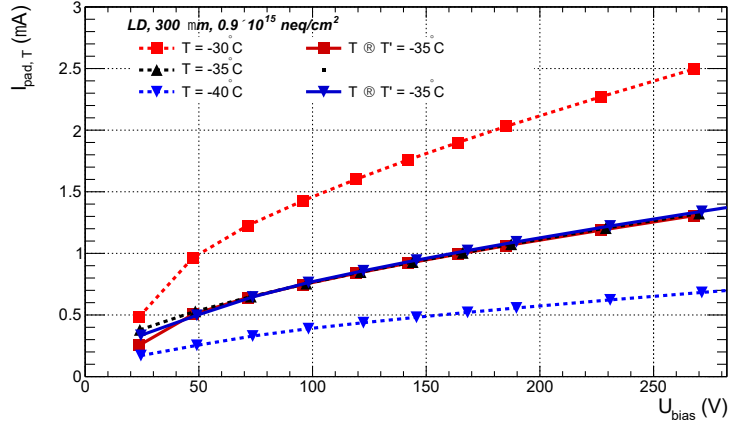
Figure 13: Leakage currents as a function of the bias voltage for an example sensor measured at -40\text{ }^{\circ}\text{C} , -35\text{ }^{\circ}\text{C} , -30\text{ }^{\circ}\text{C} , and scaled to -35\text{ }^{\circ}\text{C} using Equation (B.1).
