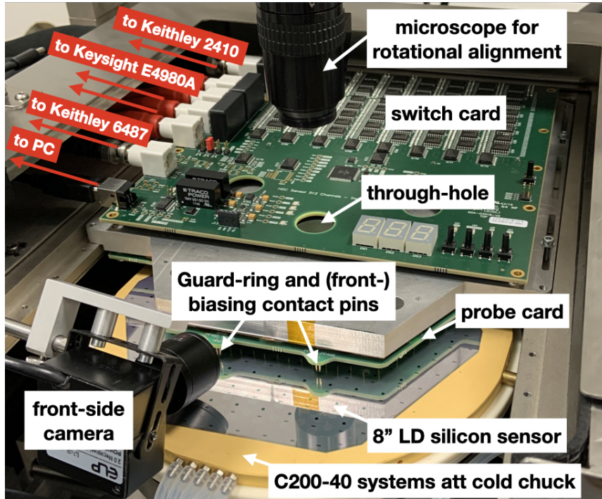
Figure 5: A low-density CE silicon pad sensor right before connecting to the switch- and probe-card ARRAY system at CERN. The probe station was closed and continuously flushed with dry air during the testing to prevent the formation of ice during low-temperature operation.
