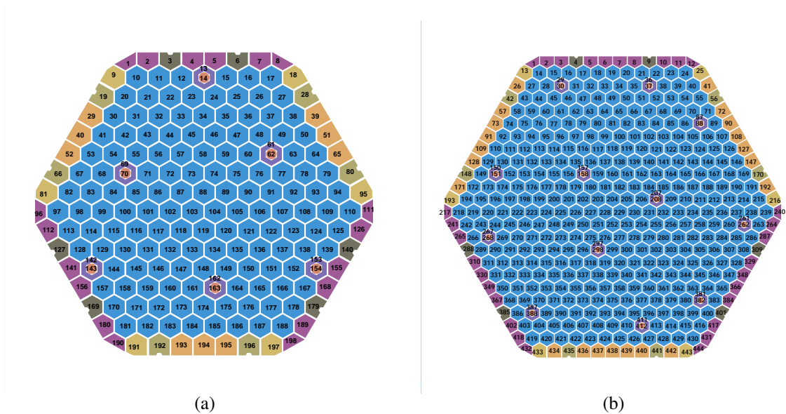
Figure 1: Layout of the tested 8'' prototype silicon pad sensors with (a) the low-density (LD) and (b) the high-density (HD) design. Regular-sized hexagonal pads are depicted in cyan. Edge and corner pads populate the sensor periphery. Six (LD), respectively twelve (HD), regular, small hexagonal pads on the sensor are dedicated for energy calibration with minimum ionising particles up to the end of life. The colour coding highlights the usage of different pad geometries. The sensor guard rings are not shown.
