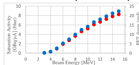
Figure 1: Saturation yield of ^{18}\text{F} (blue) and PET doses (red) as a function of E_b (saturation time of 3.5 T_{1/2} = 6.4 h).
